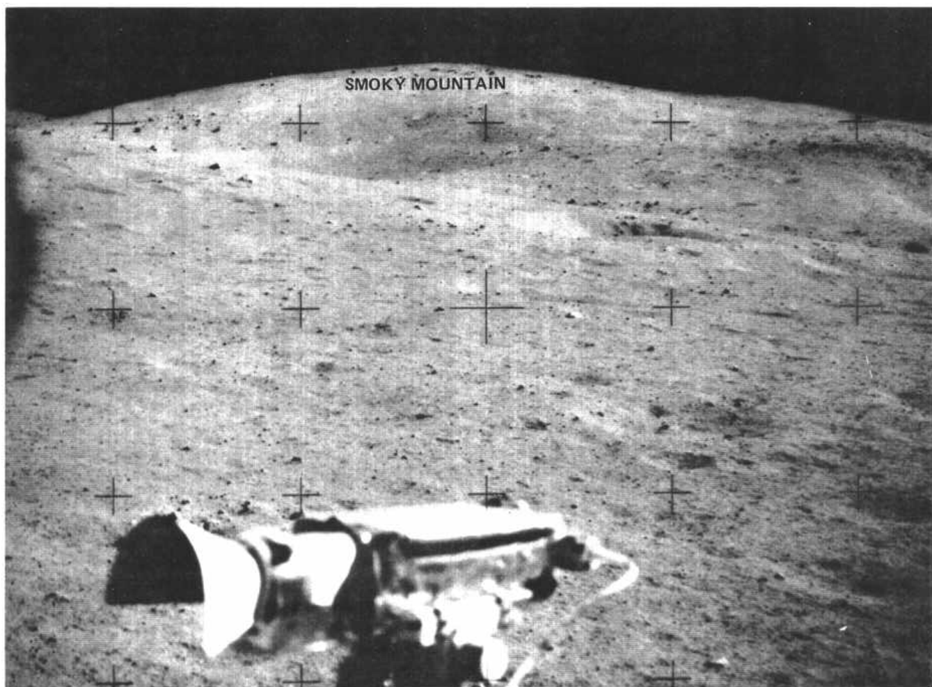
FIGURE 3.-Comparison of old and young ray-covered areas. A, Area of old ray deposit 1.5 km from rim of North Ray crater AS16- 111-14143, view is northeast. B, Area of young ray deposit 4.5 km from rim of South Ray crater. AS16-110-17898, view south.
