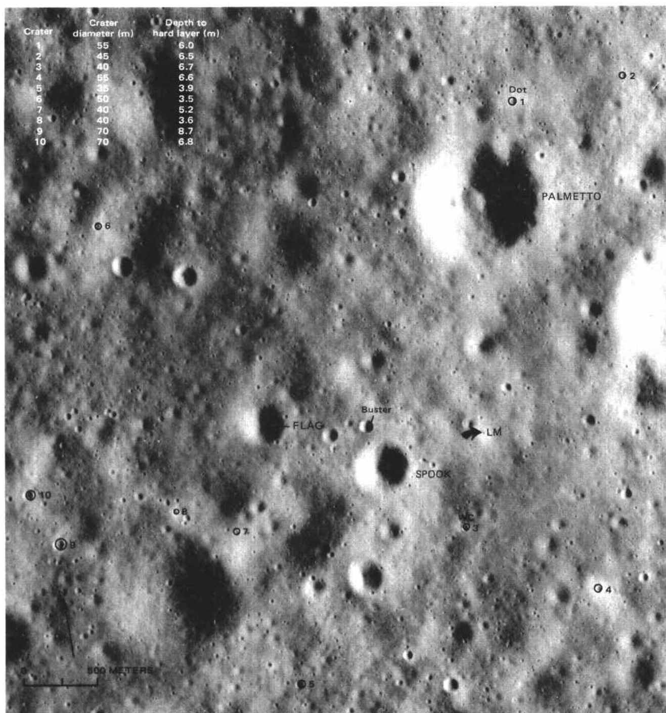
FIGURE 4.-Locations of concentric craters used to estimate depth of regolith. Apollo 16 panoramic camera frame 4623.
