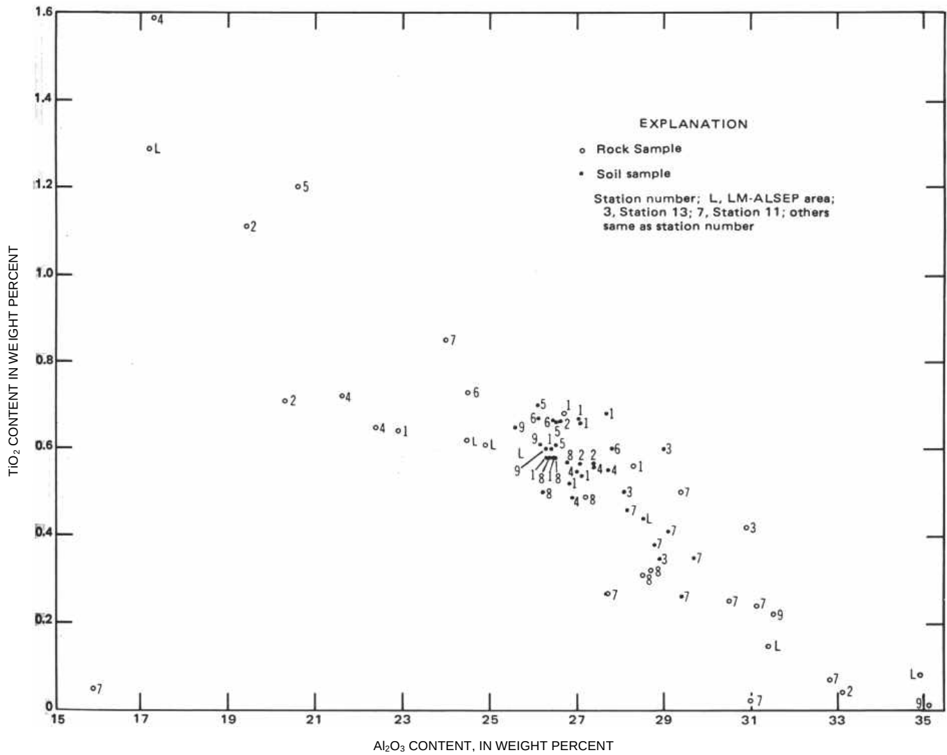
FIGURE 7.-Plot of \text{TiO}_2 relative to \text{Al}_2\text{O}_3 , for rock and soil samples. Points are averages of all available analyses of each sample.
