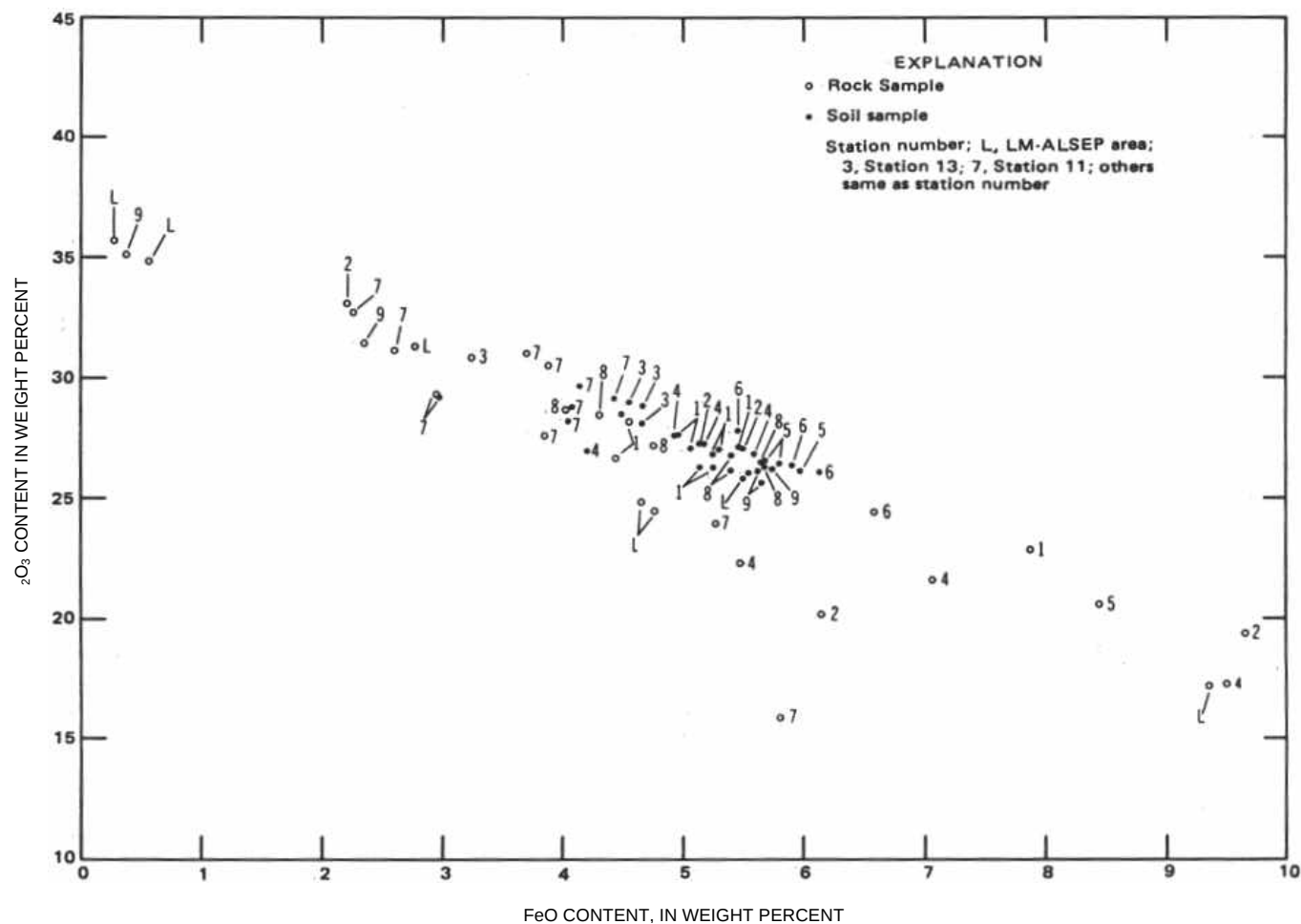
FIGURE 8.-Plot of \text{Al}_2\text{O}_3 relative to FeO of rock and soil samples. Multiple analyses of same samples are averaged.
