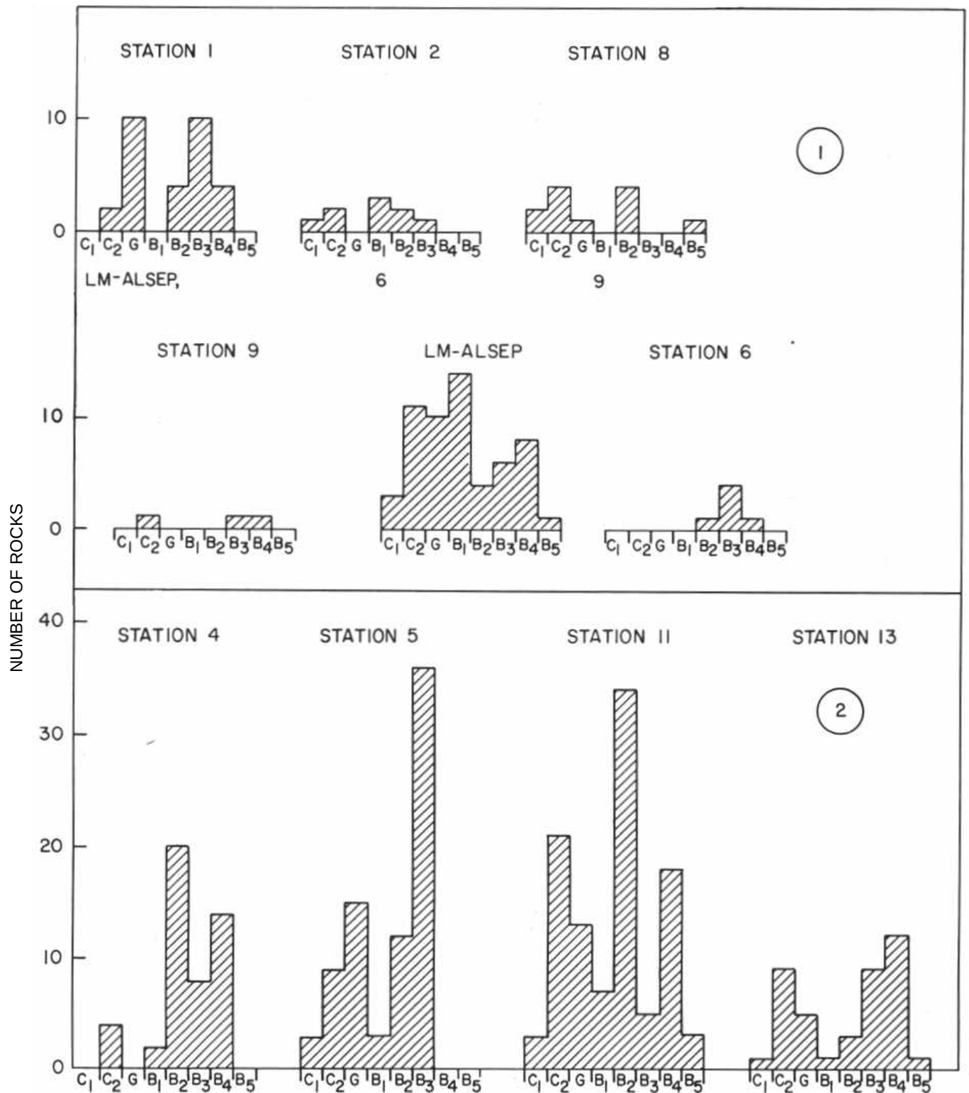
FIGURE 5.-Histograms showing distribution of rock types at each sampling station. Rocks in group 1 are from Cayley plains, those in group 2 from Descartes mountains and the ejecta blanket of North Ray crater.
