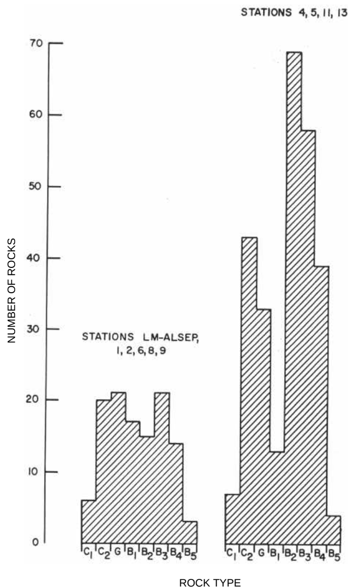
FIGURE 6.-Composite histograms of the two groups of stations.
