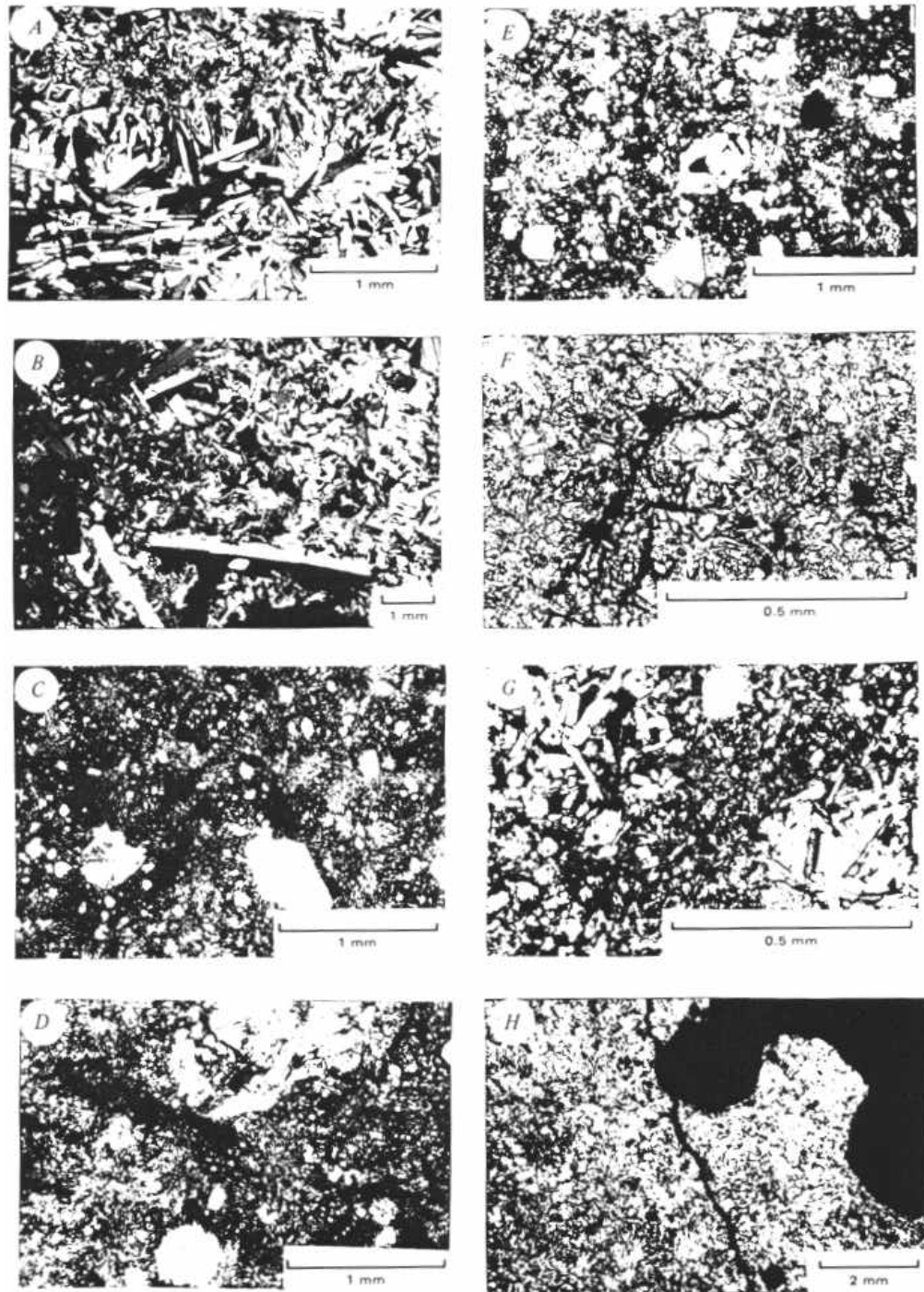
FIGURE 2.-Photomicrographs of Apollo 16 crystalline rocks and one Apollo 17 rock. A, Sample 68415 (group C 1 ), showing textural variations within an impact melt that cooled moderately slowly. Cross-polarized light. B, Sample 65055 (group C 1 ), showing inequigranular texture within an impact melt that cooled moderately slowly. Cross-polarized light. C, Sample 60616 (group C 2 ), showing fine-grained poikiloblastic texture. Mafic minerals do not interlock; areas between them have granoblastic texture. Cross-polarized light. D, Sample 60625. (group C 2 ), medium-grained poikiloblastic texture. Mafic minerals interlock; enclosed minerals dominantly very fine grained, anhedral. Cross-polarized light. E, Sample 65778 (group C 2 ), showing coarse-grained poikiloblastic texture. Mafic minerals interlock; note unusual amount of mineral debris (light color). Cross-polarized light. F, Sample 60315 (group C 2 ), showing interstitial igneous texture between large poikiloblastic orthopyroxene grains. Plane-polarized light. G, Sample 60315 (group C 2 ), showing spherical droplets with intersertal to intergranular igneous texture in coarse-grained poikiloblastic rocks. Plane-polarized light. H, Apollo 17 sample 76215, showing transition from poikiloblastic texture (left) in which orthopyroxene oikocrysts enclose abundant mineral debris to ophitic texture with polkilitic clinopyroxene and less mineral debris. Vesicles occur only in the ophitic area. Cross-polarized light.
