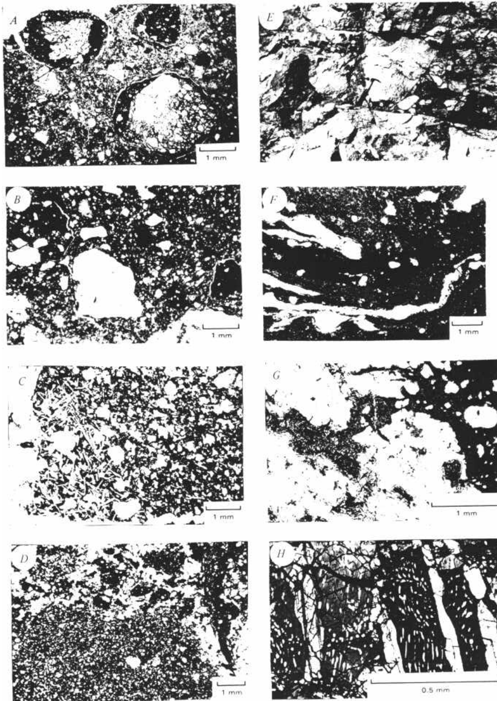
FIGURE 4.-Photomicrographs of Apollo 16 breccia photograph and photo micrographs of pseudotachylites of Vredefort structure. South Africa, E-G. A, Sample 67035 (B 2 breccia), showing clasts with selvages embedded in a friable light-gray matrix containing a variety of lithic and mineral microclasts. Plane-polarized light. B, Sample 61295 (B 3 breccia), showing a variety of clasts, including glass, in a fine-grained glassy matrix. Plane-polarized light. C, Sample 60018 (B 4 breccia), showing a cataclastic anorthositic clast at one edge grading into an impact melt zone with ophitic texture, and this into intersertal texture. Plane-polarized light. D, Sample 68815 (B 5 breccia), showing a small area in a rock dominated by dark clasts in dark matrix. This area shows a remnant of B 2 breccia with feldspathic debris in fractures in the fine-grained dark original matrix. Plane-polarized light. E, Pseudotachylite, Vredefort structure, South Africa, showing breccia composed of clasts of crystalline rock in finely comminuted and locally fused material of the same chemical composition as the clasts. Photograph by Warren Hamilton. F, Pseudotachylite in alkali granite, Vredefort structure, South Africa, showing cataclastic flow structures in comminuted alkali granite, metamorphosed to very fine grained granoblastic texture. Cross-polarized light. G, Pseudotachylite in Old Granite, Vredefort structure, South Africa; local fused zone showing newly crystallized feldspar laths and flow structure. Cross-polarized light. H, Sample 62236 (B 4 breccia), showing coarse irregular and finer regular clinopyroxene exsolution lamellae (white) in orthopyroxene (dark). Cross-polarized light.
