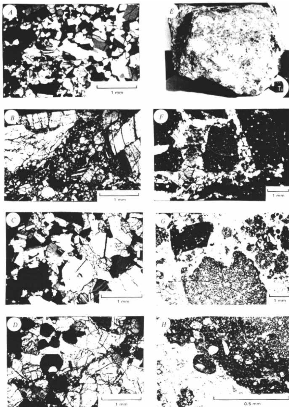
FIGURE 3 -- Photomicrograph of Apollo 16 metaclastic rock and breccias and photograph of breccia 61015. A. Sample 60619 (group C 2 ), showing coarse hornfels texture in metaanorthosite. Cross-polarized light. B. Sample 62237 (B 1 breccia), showing coarse mineral relics and cataclastic flow structure in troctolite. Cross-polarized light. C. Sample 65785 (group C 2 ), a lithic relic in cataclasite, having postcumulus olivine (high relief) separating cumulus plagioclase grains twinned. Cross-polarized light. D. Sample 67435 (B 4 breccia), showing lithic clast in breccia with postcumulus plagioclase (low relief, white) separating cumulus olivine (high relief) and spinel (in extinction) grains. Cross-polarized light. E. Sample 61015 (NASA photograph S-72-40585B), showing net-veining of original dark matrix by clastic material derived from the white clasts. F. Sample 61015 (B 2 breccia), showing weakly annealed, coarse mineral debris in fractures in original matrix (dark). Cross-polarized light. G. Sample 66055 (B 2 breccia), showing glass selvage (dark gray) on lighter gray fragment of original matrix. Note surrounding fragments of spalled selvage in feldspathic debris derived from original clasts. Plane polarized light. H. Sample 66055 (B 2 breccia), showing incompletely spalled ellipsoid of glass selvage. Plane-polarized light.
