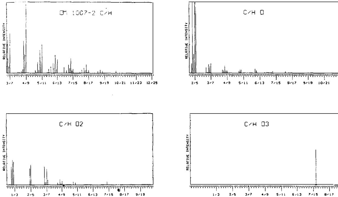
Figure C-2. - Mass spectrometer scans for organic monitor 1007-2.
