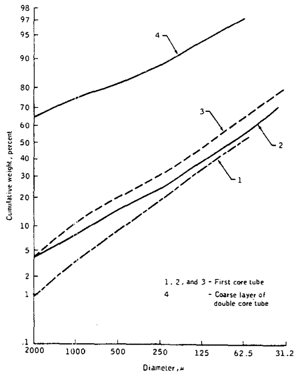
Figure A-21. - Mechanical analyses of first core tube and of coarse layer of double core tube.
