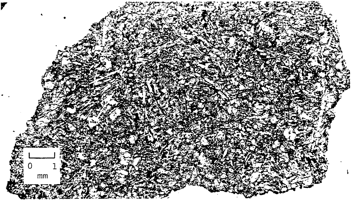
Figure A-64. - Sample 12002-7 (NASA-S-70-31576).
