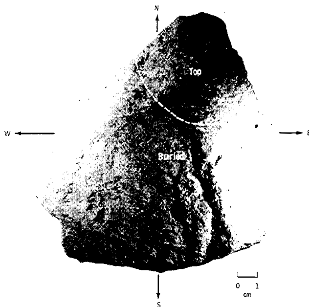
(g) Suggested selenographic orientation of sample 12022 (NASA-S-69-61999).
