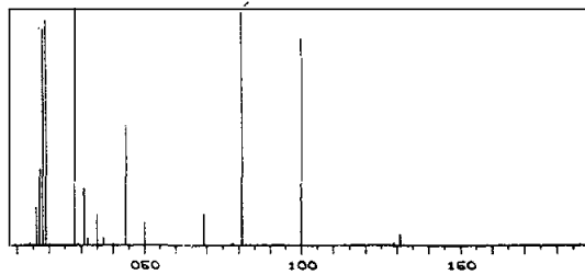
Figure B-9. - Mass spectrometer scans for sample 12034-2.
