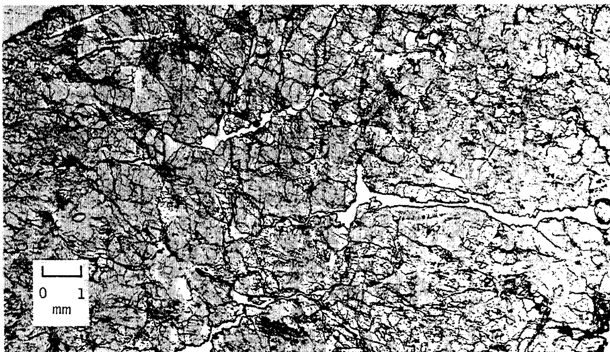
Figure A-85. - Sample 12057-14 (NASA-S-69-64831).
