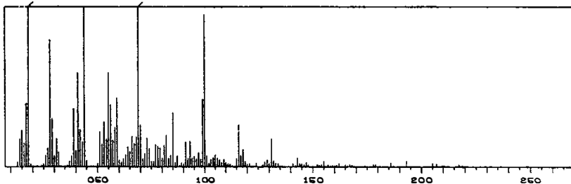
Figure B-13. - Mass spectrometer scans for sample 12059-1.
