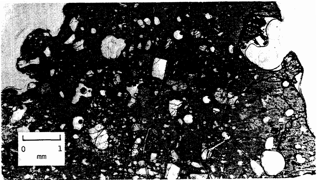
Figure A-89. - Sample 12057-22 (NASA-S-69-63404).
