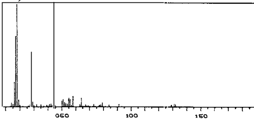
Figure B-8. - Mass spectrometer scans for sample 12028-1.
