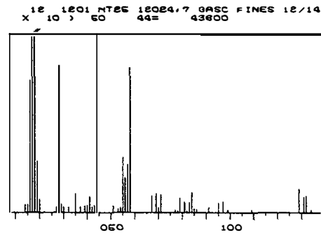
Figure B-3. - Mass spectrometer scans for sample 12024-7, run 1.
