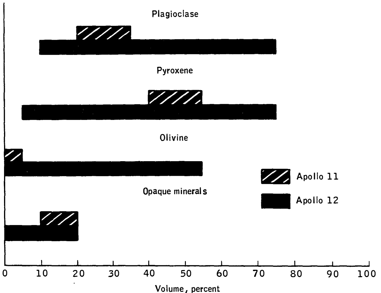
Figure 7. - Apollo 11 and 12 lunar-sample modal analyses.
