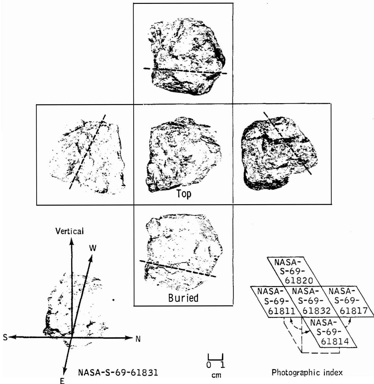
(b) Suggested selenographic orientation of sample 12031.
