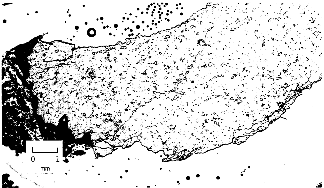
Figure A-66. - Sample 12008-15 (NASA-S-70-44572).
