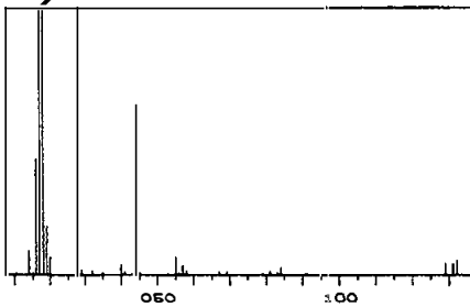
Figure B-12. - Mass spectrometer scans for sample 12057-1.
