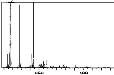
Figure B-2. - Mass spectrometer scans for sample 12003-1.
