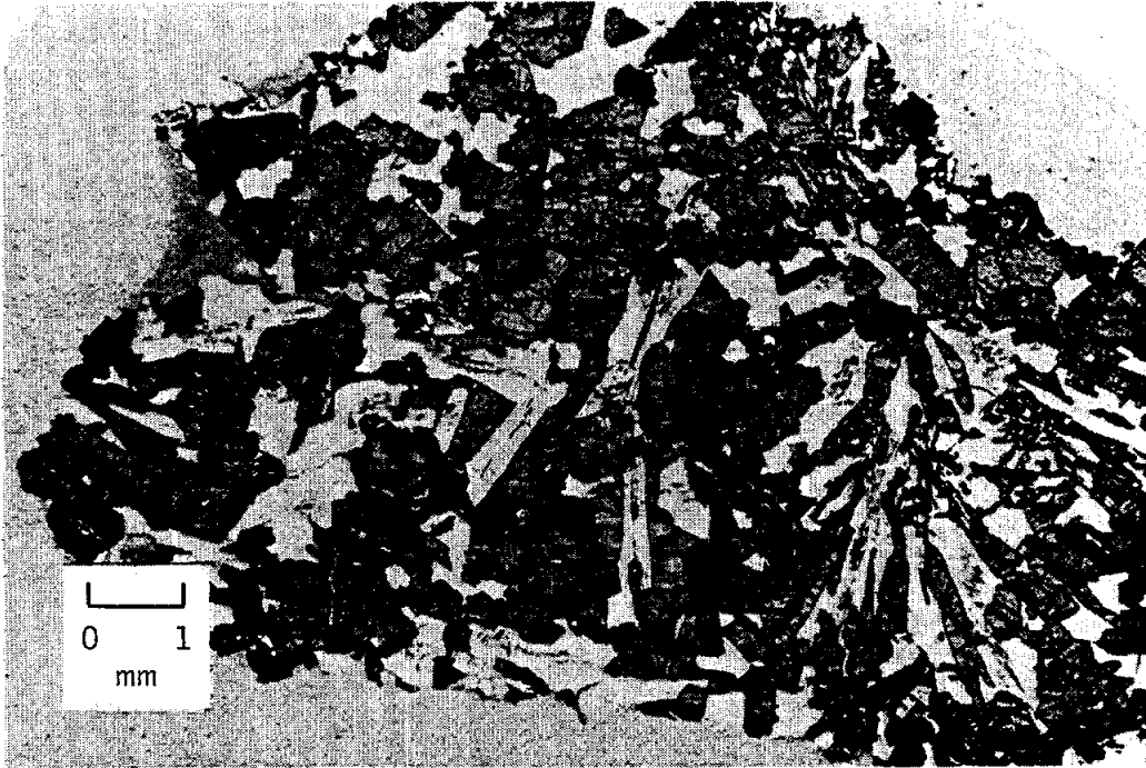
Figure A-80. - Sample 12040-3 (NASA-S-69-24211).
