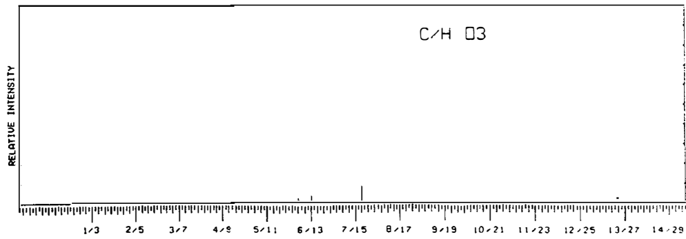
Figure C-7. - High-resolution mass-spectral data for benzene.
