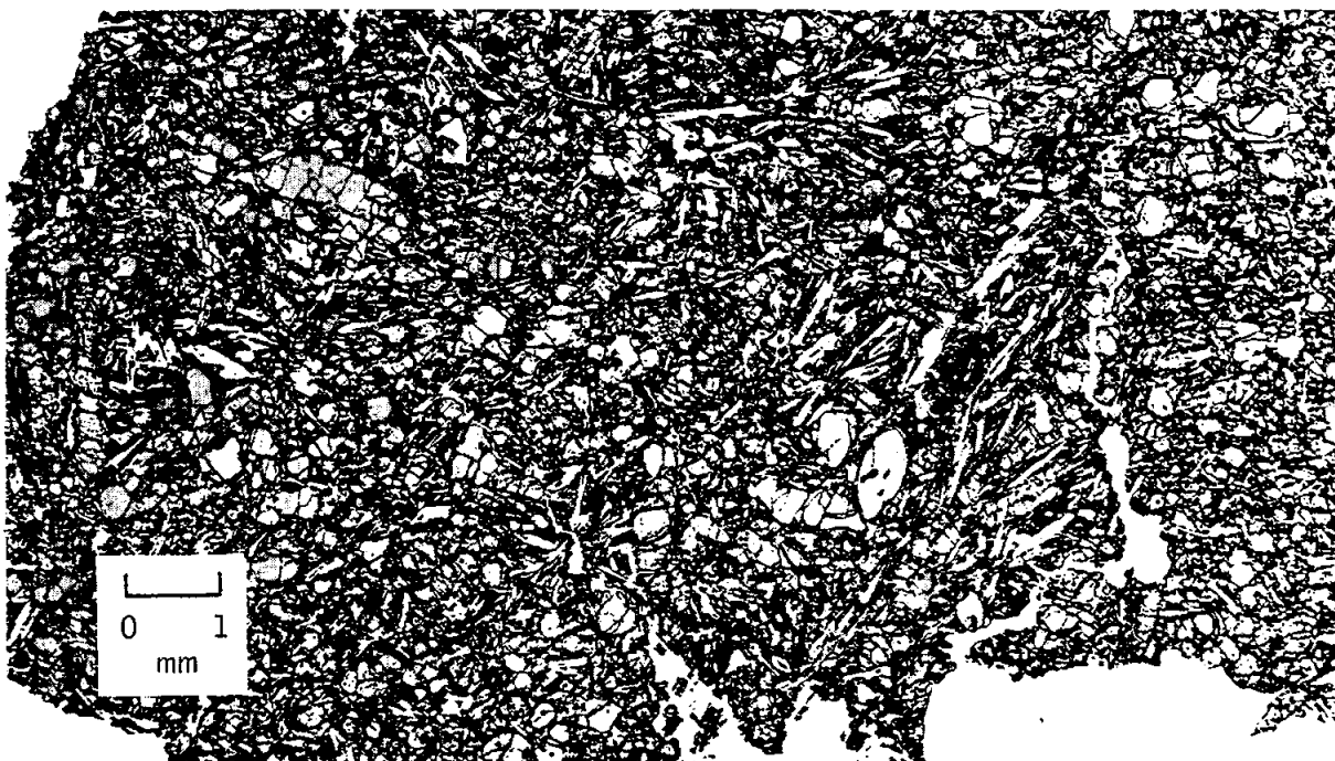
Figure A-69. - Sample 12012-5 (NASA-S-69-24220).
