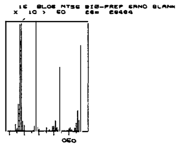
Figure B-1. - Mass spectrometer scans for control sample 1201.
