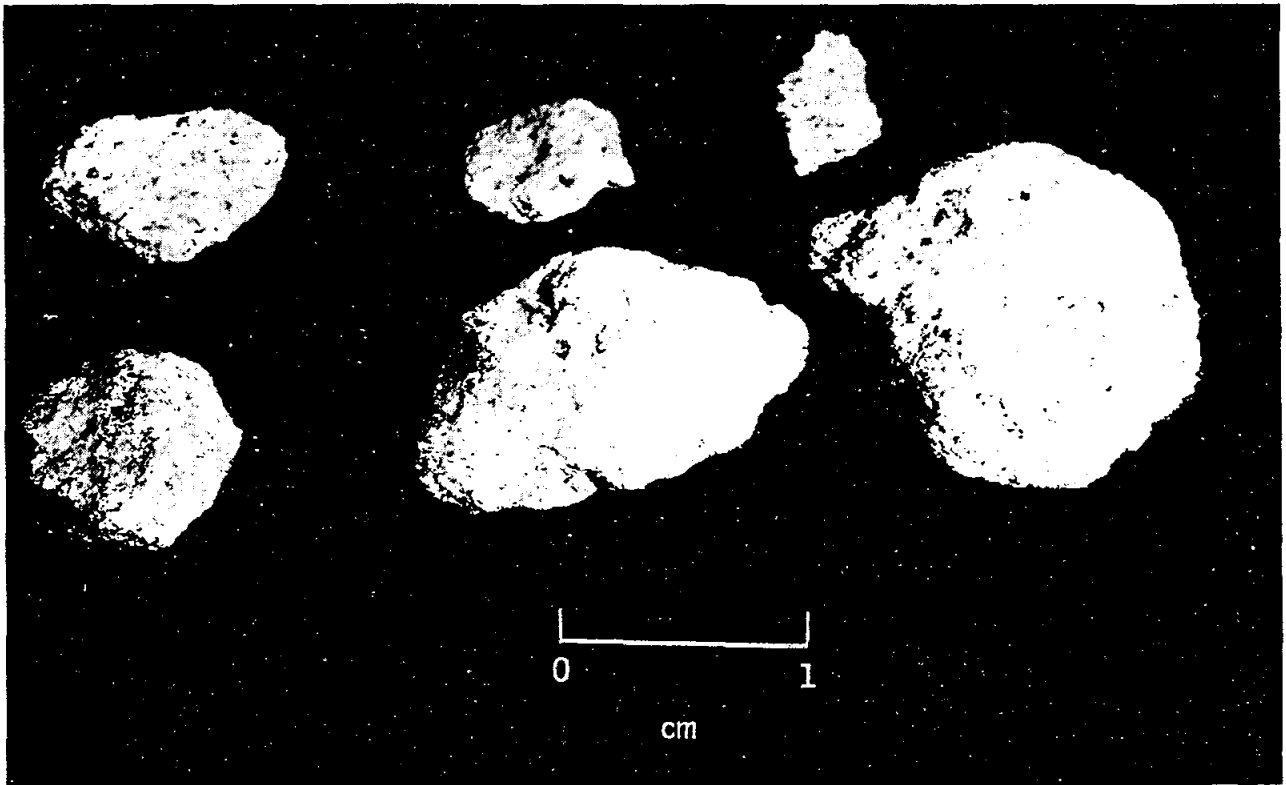
Figure A-53. - Sample 12061 (NASA-S-69-61659).
