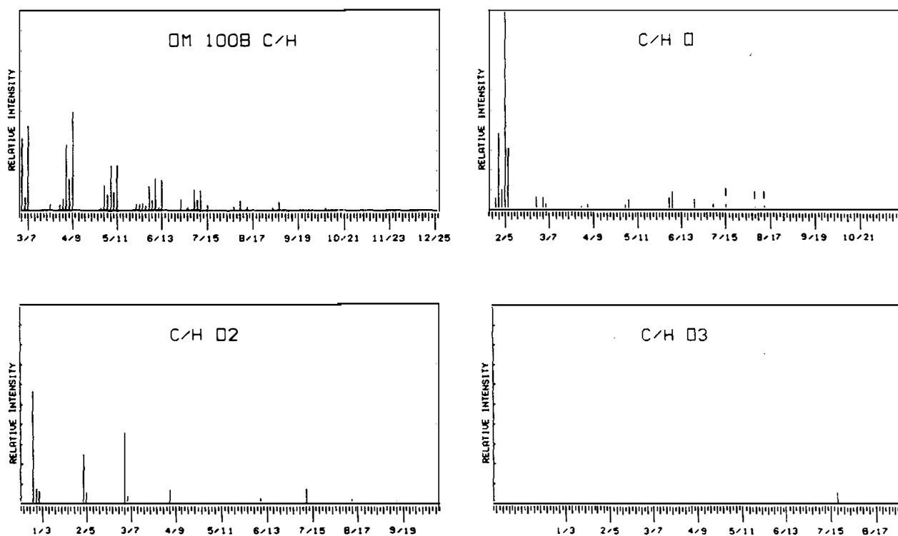
Figure C-4. - Mass spectrometer scans for organic monitor 1008.
