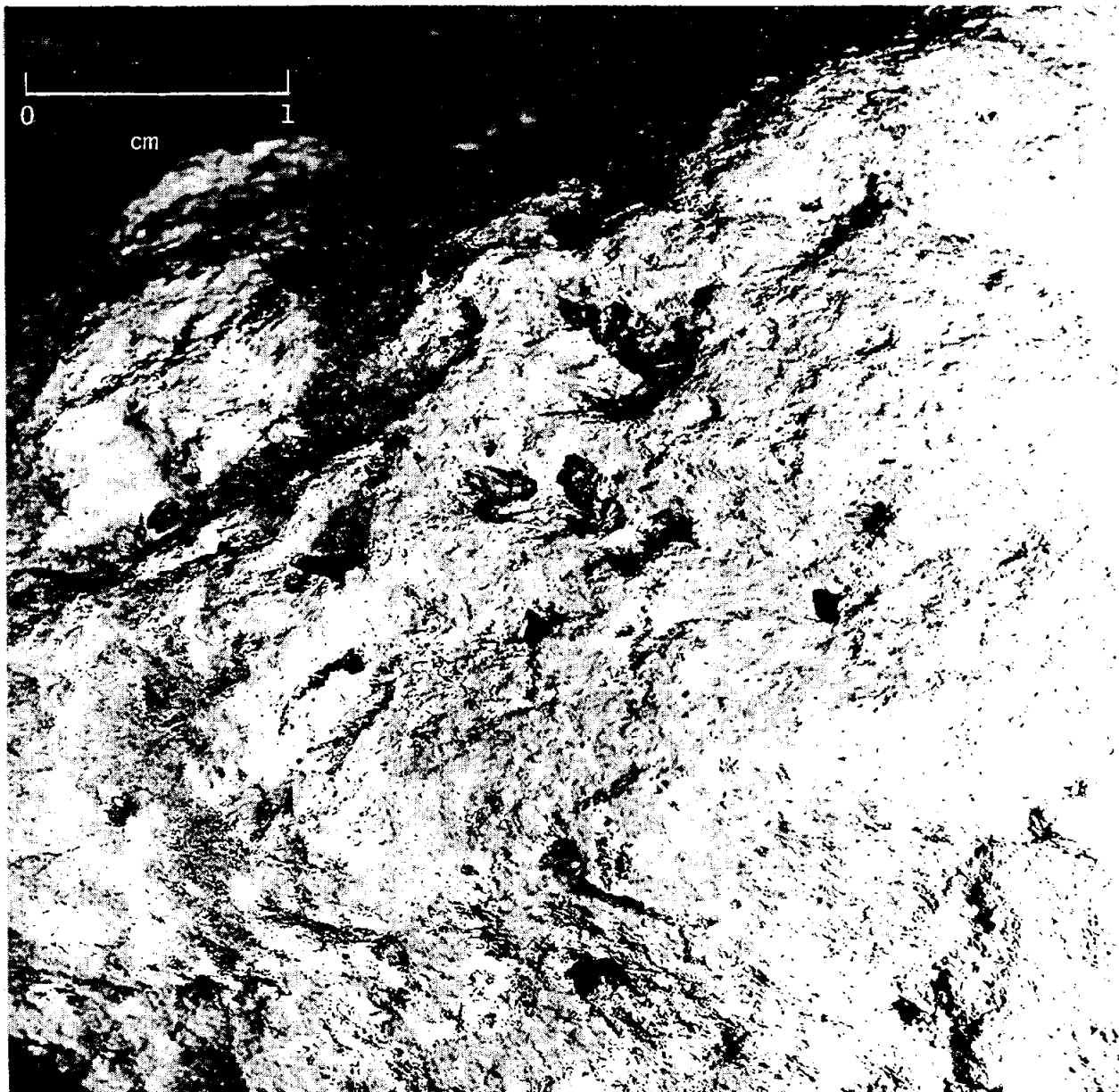
Figure A-38. - Closeup of sample 12052 (NASA-S-70-21312).
