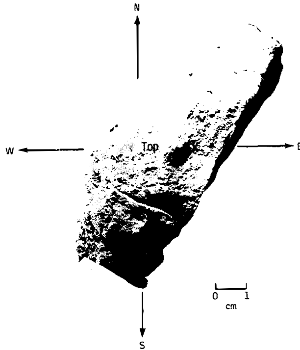
(b) Suggested selenographic orientation of sample 12004 (NASA-S-69-62023).
