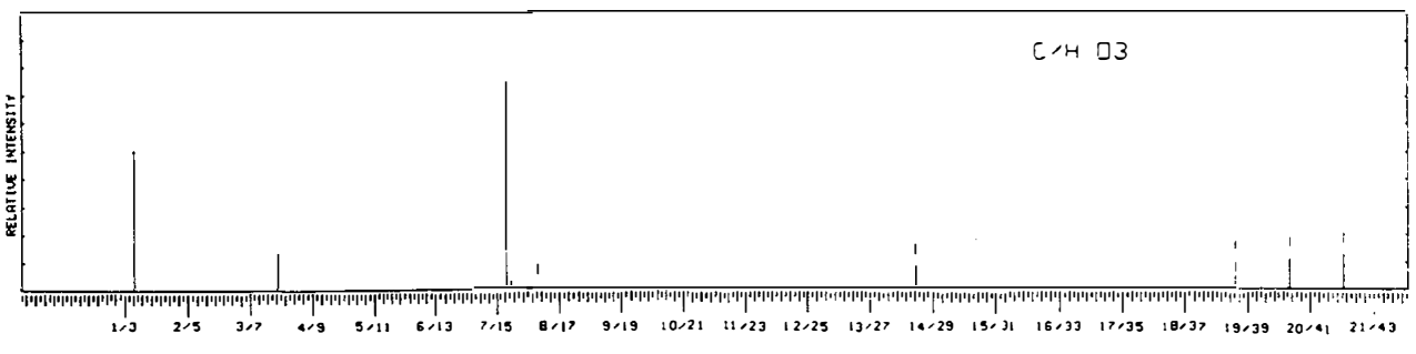
Figure C-5. - Mass spectrometer scans for organic monitor 1009.
