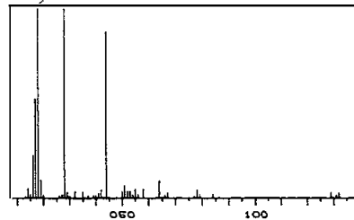
Figure B-8. - Mass spectrometer scans for sample 12028-1.
