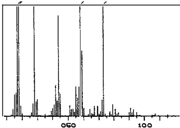
Figure B-13. - Mass spectrometer scans for sample 12059-1.
