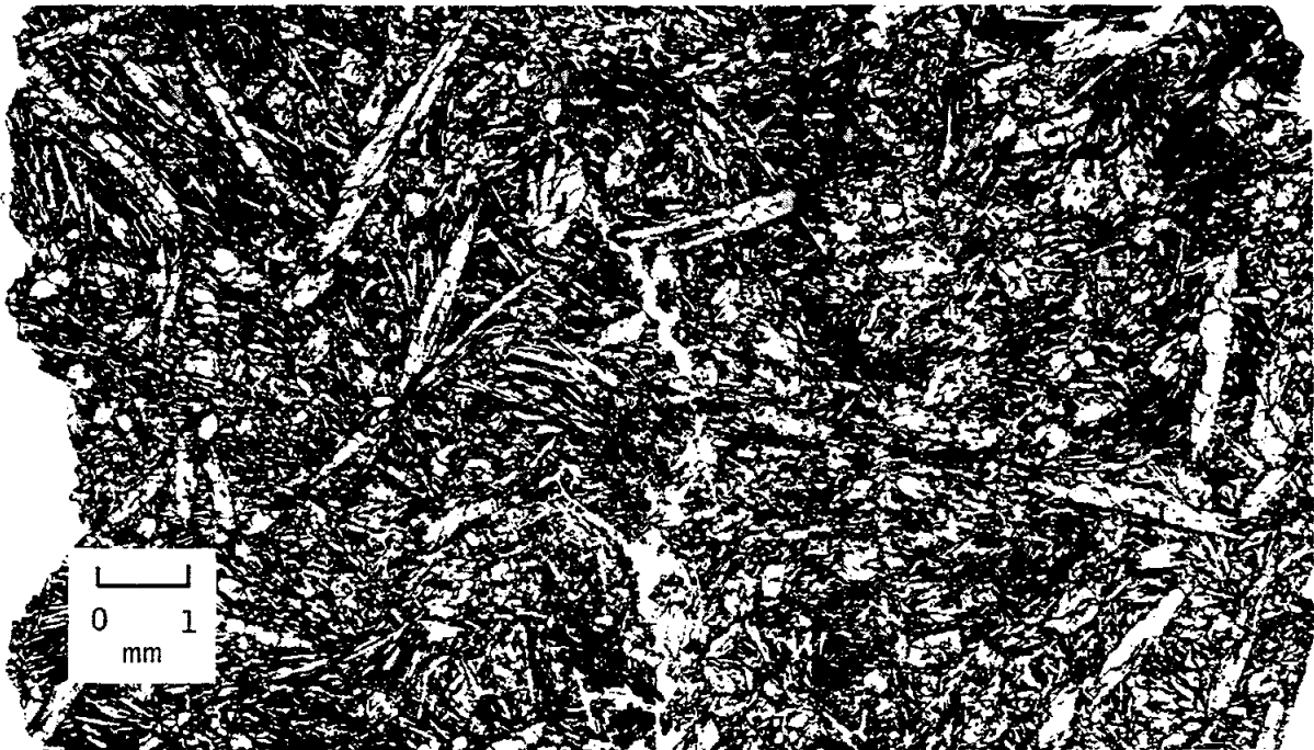
Figure A-93. - Sample 12065-6 (NASA-S-69-23378).
