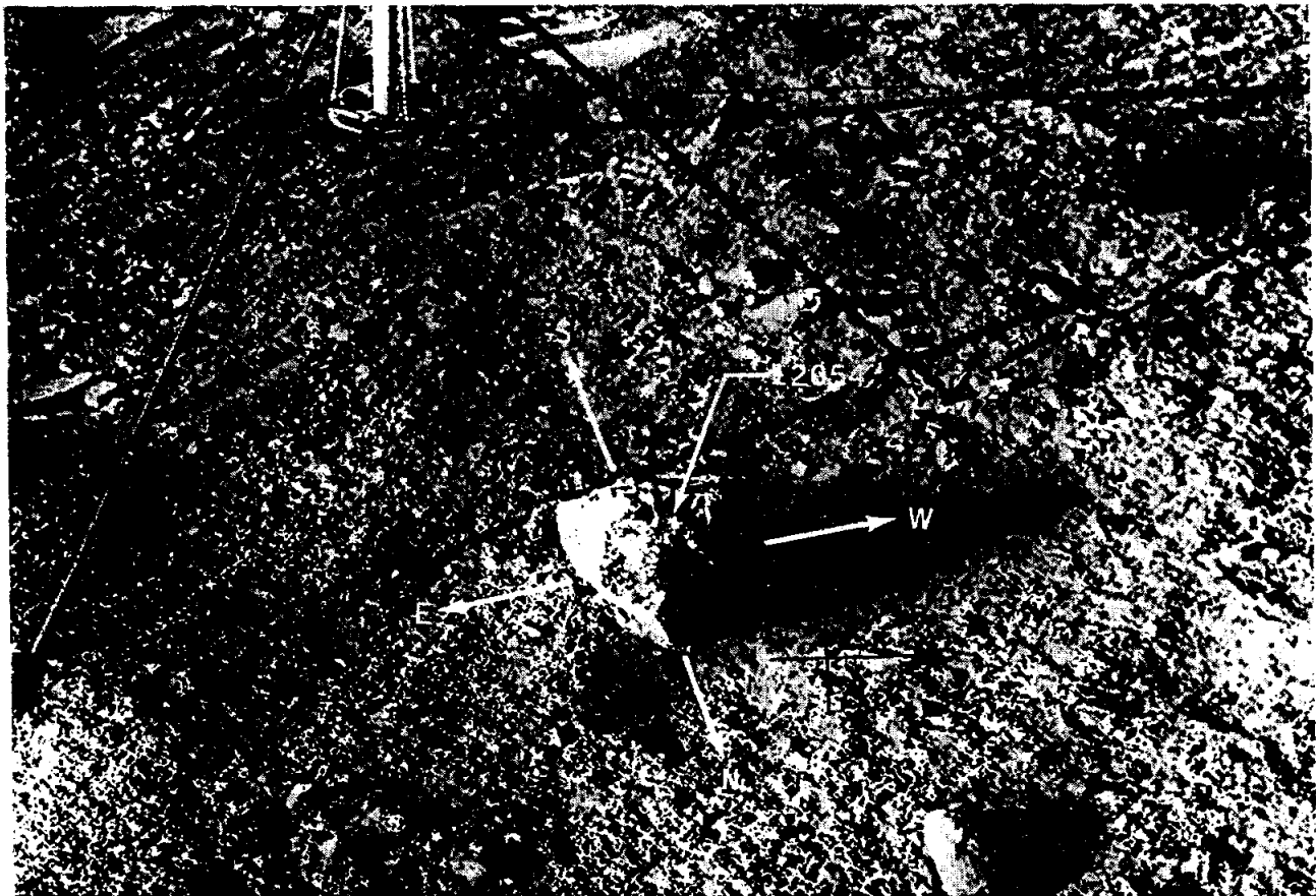
(h) Sample 12054 before collection (AS12-49-7315).
