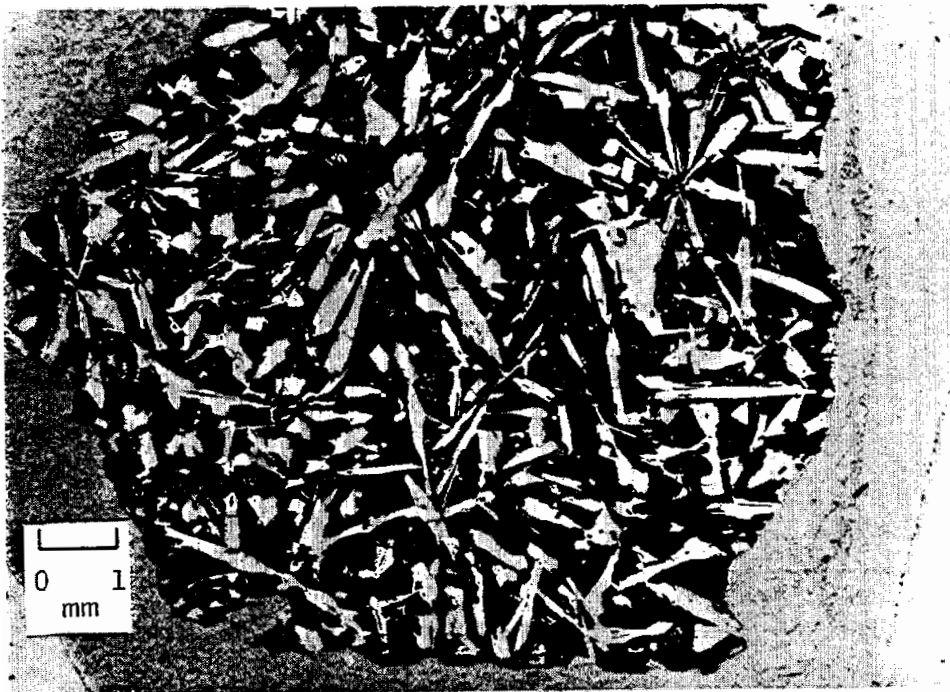
Figure A-79. - Sample 12038-2 (NASA-S-69-24203).
