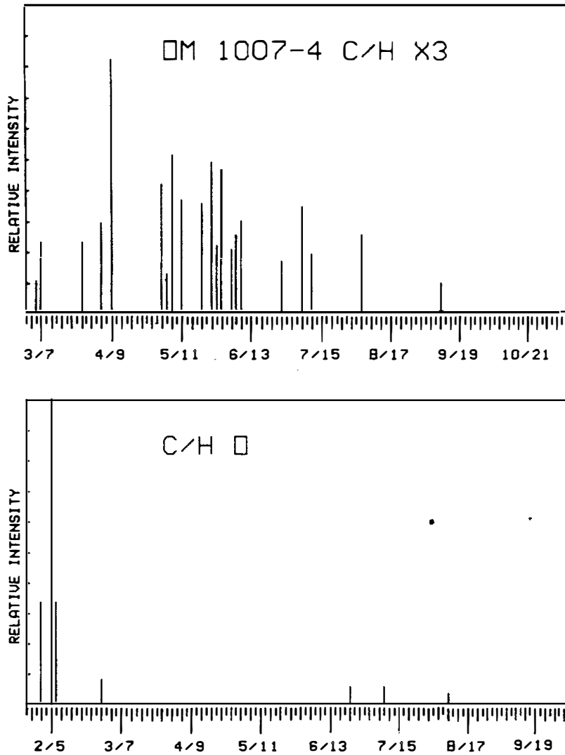
Figure C-3. - Mass spectrometer scans for organic monitor 1007-4.
