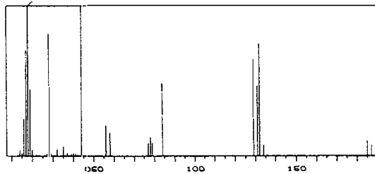
Figure B-11. - Mass spectrometer scans for sample 12052-4.
