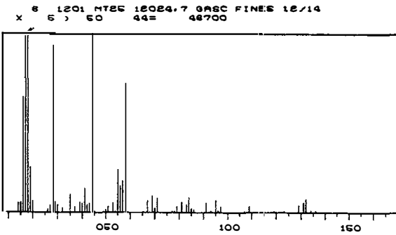
Figure B-3. - Mass spectrometer scans for sample 12024-7, run 1.
