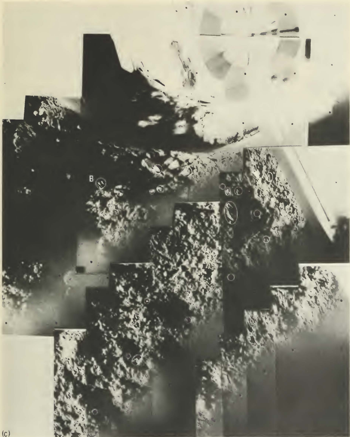
FIGURE 4-29.—Continued. (c) Mosaic of the same pictures used in figure 4-29(b); however, the fragments circled are those fragments shown by later pictures to have been moved by the 60-second attitude control jet firing (Nov. 9, 1967, Catalog 6-MP-2).
