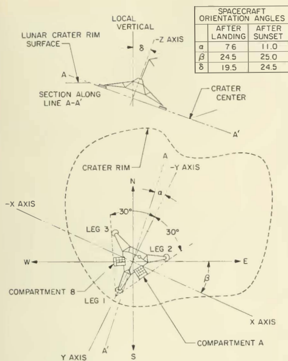
FIGURE 6-25.—Surveyor VI landed orientations.
