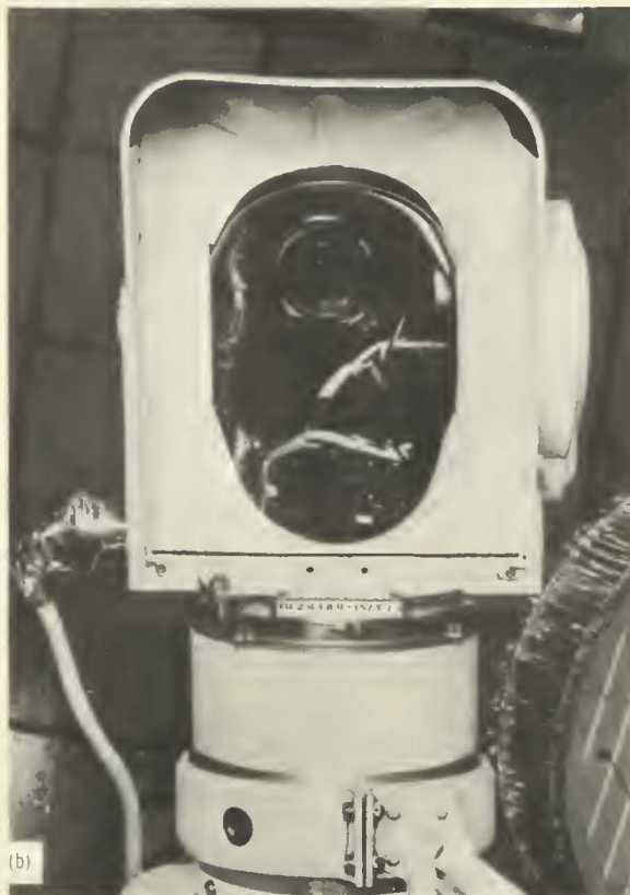
FIGURE 3-2.—Mirror assembly of the Surveyor television camera. (a) Surveyor I television camera hood and mirror assembly. A small visor was added to the top of the hood on the Surveyor III camera. (b) Mirror assembly and redesigned hood used on Surveyors V, VI, and VII.
