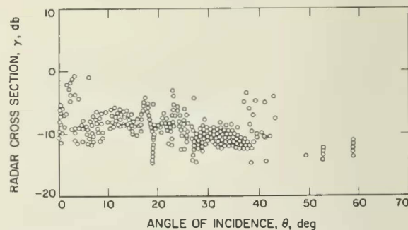
FIGURE 7-12.—Radar cross section for Surveyor VII as a function of incidence angle. All beams are superimposed.
