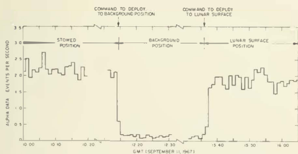
FIGURE 8-21.—Plot of event rate of analyzed alpha particles as a function of time, showing marked decrease when the Surveyor V sensor head was deployed from the stowed to the background position and the increase when lowered from the background position to the lunar surface.
