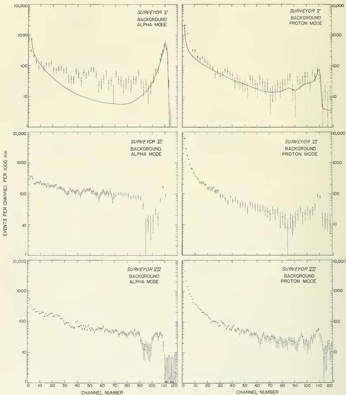
FIGURE S-32.—Surveyor V, VI, and VII background measurements on the Moon. Parts of the Surveyor V and VI data are the averages of two channels. The smooth curves in the Surveyor V graphs are the premission predictions of the background rates.
