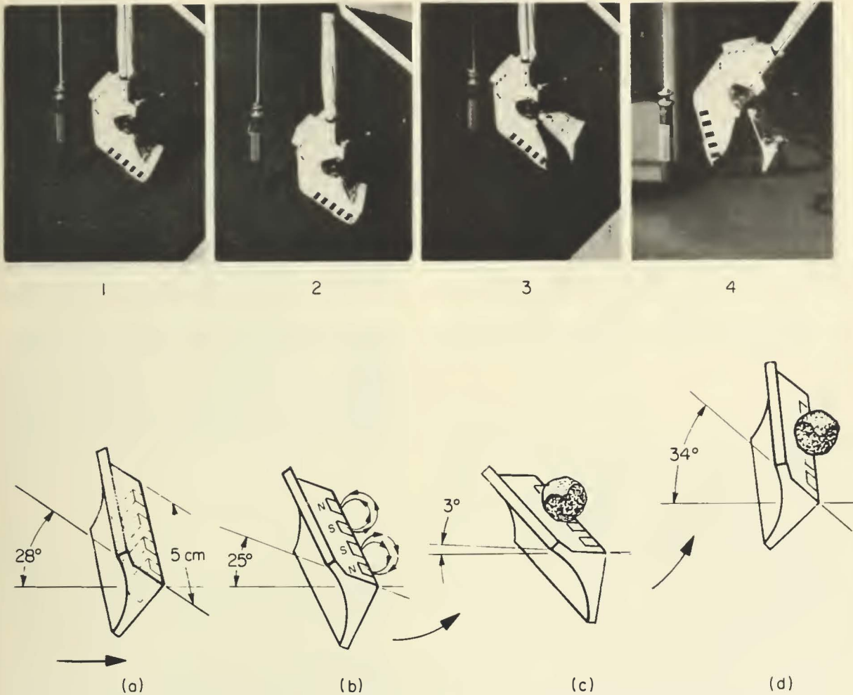
FIGURE 7-36.—Concluded. (j) Laboratory simulation of angular relationships of surface-sampler magnets to the lunar surface during pickup of magnetic fragment. Note plumb bob.
