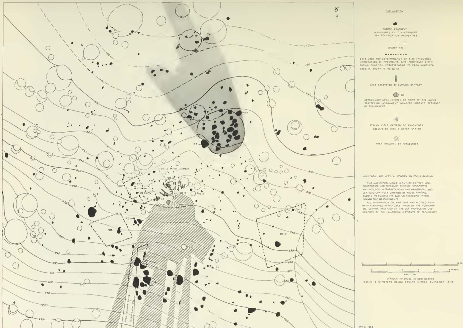
FIGURE 3-25.—Contour map (by Raymond Jordan) of the near field of the Surveyor VII landing site. The map was made from focus-ranging data.
