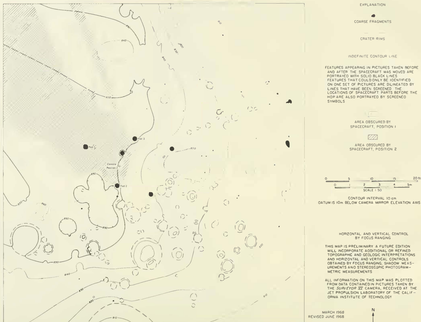
FIGURE 3-24.—Contour map (by Raymond Jordan) of the near field of the Surveyor VI landing site. The map was made from focus-ranging surveys taken both before and after the hop. Features that could be identified on one set of pictures only (taken either before or after the hop) are shown with shaded lines, as are the locations of spacecraft parts before the hop. All other features are shown with solid lines.
