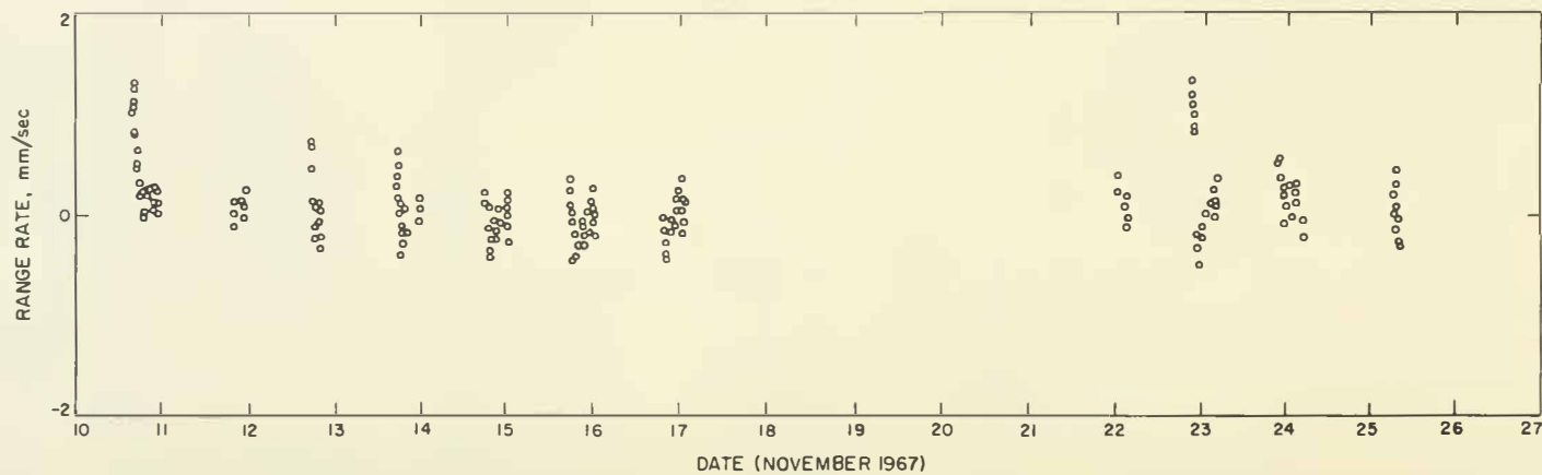
FIGURE 10-27.—Surveyor VI, DSS 61. First lunar day, O—C residual set (compressed five data points/min). LE 5 was used.
