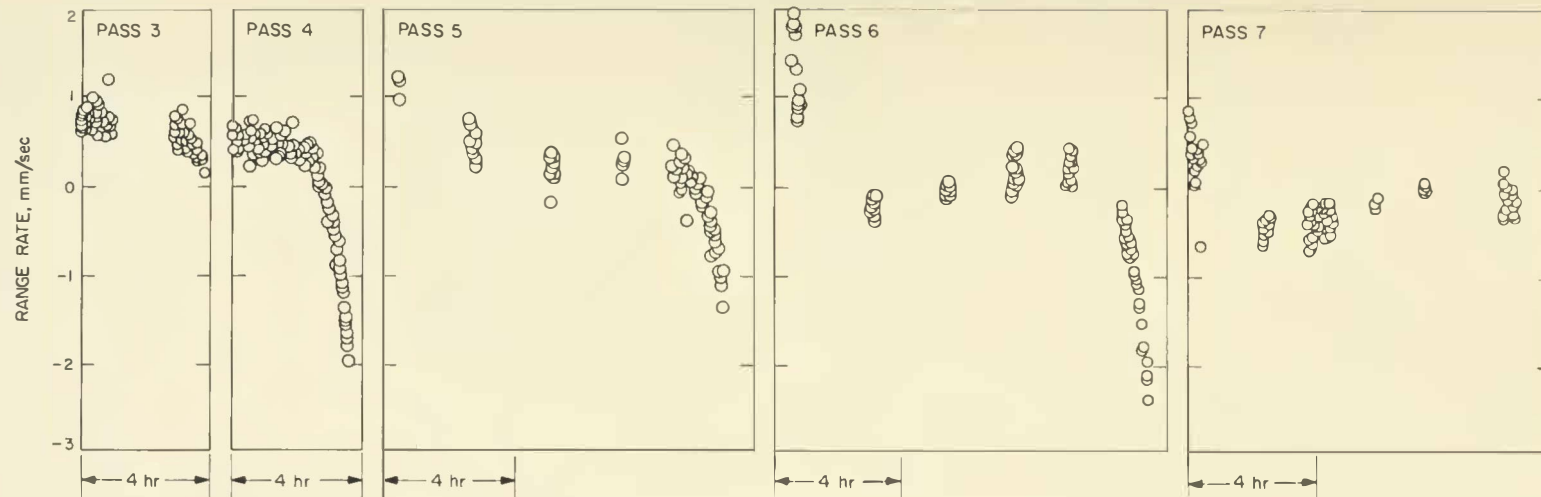
FIGURE 10-28.—Surveyor VI. Tracking passes of unbiased and biased data: DSS 11.
