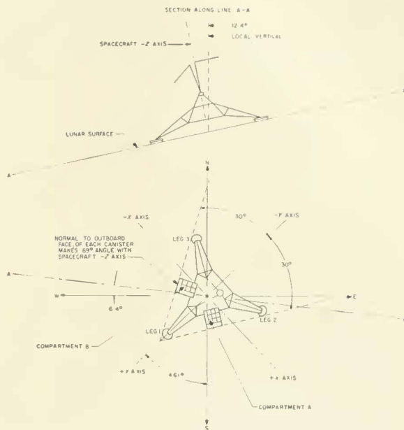
FIGURE 6-21.—Surveyor III landed orientation.
