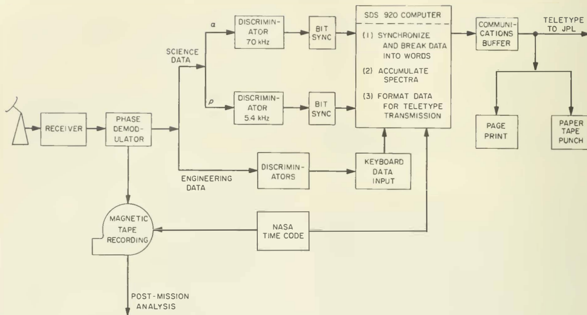
FIGURE 8-17.—Alpha-scattering data processing system at the Deep Space stations.
