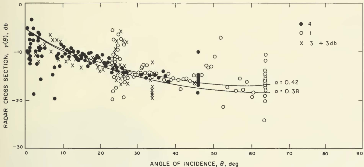
FIGURE 7-20.—Radar cross section versus angle of incidence for Surveyor VI. F_2(\theta) scattering model, with \alpha=0.38 and 0.42 .
