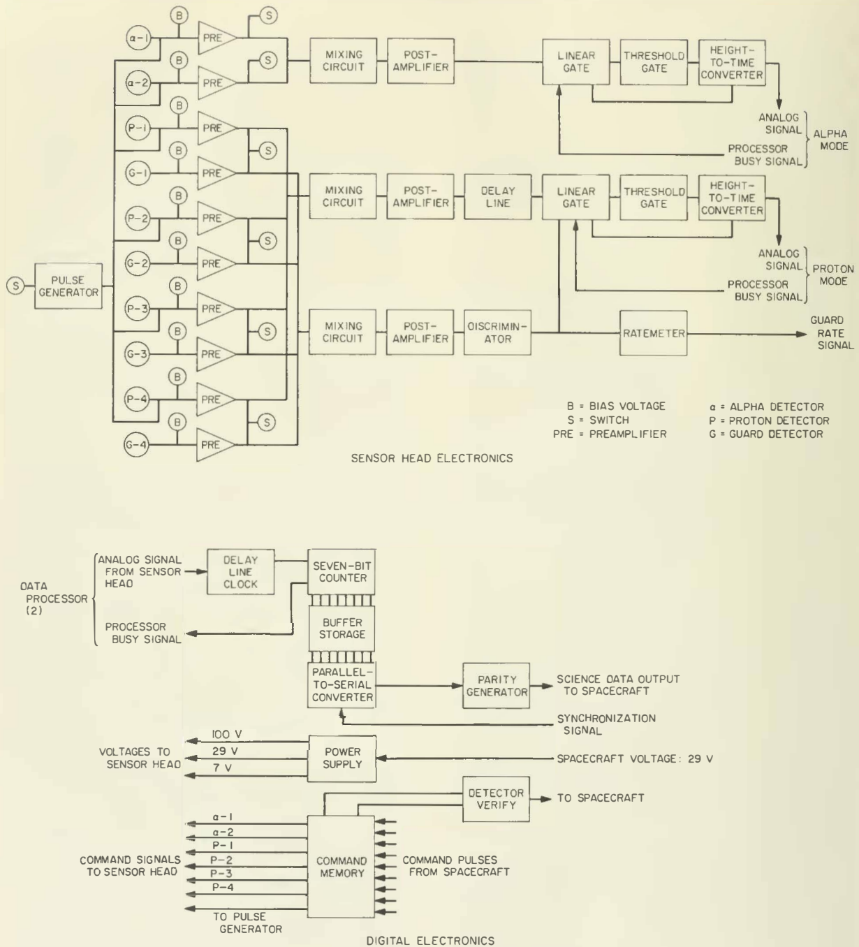
FIGURE 8-12.—Block diagram of the electronic circuitry contained in the alpha-scattering instrument.
