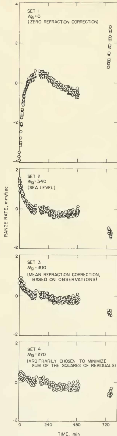
FIGURE 10-9.—Surveyor VII. Pass 11 for DSS 61. Refraction influence on SPODP residuals. LE 5 was used.
