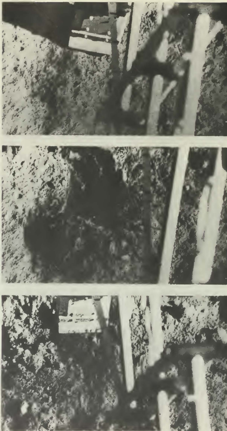
FIGURE 7-29.—Views of the surface-sampler magnets, before, during, and after the first bearing strength test. The depth of the test was about 5 cm. Some magnetic material can be seen around the magnetic pole ends. (See fig. 7-33 for test area.)
