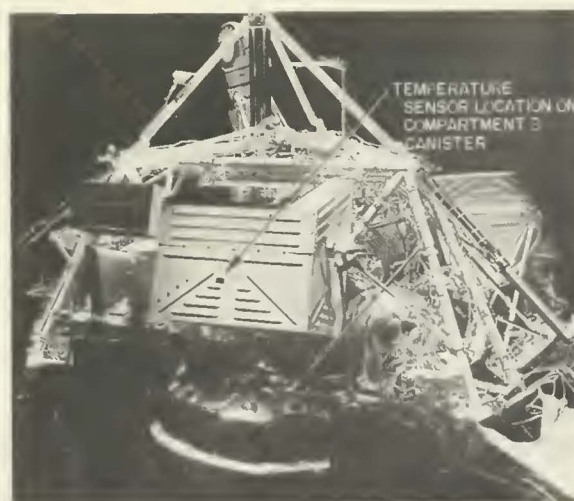
FIGURE 6-17.—Surveyor model, compartment B.
