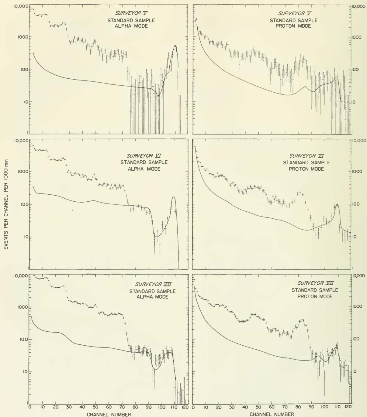
FIGURE S-29.—Surveyor V, VI, and VII standard sample measurements on the Moon. The experimental points (crosses) are indicated with statistical ( 1\sigma ) error bars. The solid curves are smoothed versions of the background spectra observed in the next stage of lunar operations.
