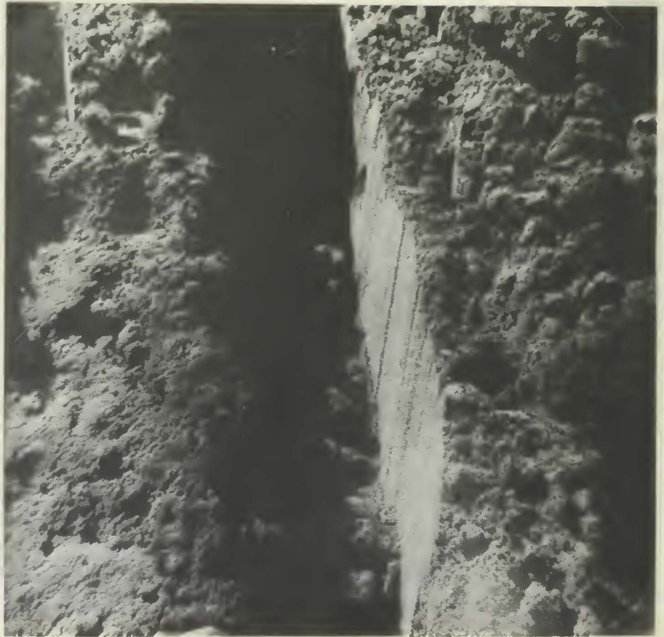
FIGURE 7-43.—Concluded. (e) Surveyor VII. Top: imprint of footpad 2; bottom: closeup of a trench wall. All trench walls showed a similar smooth texture (see fig. 7-33).
