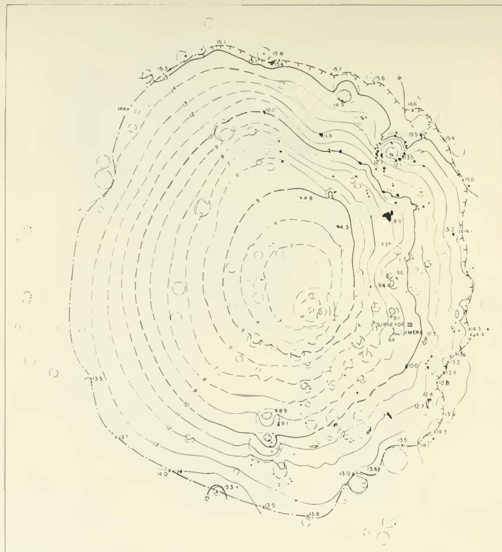
FIGURE 3-19.—Contour map of the Surveyor III landing site. Contour lines were drawn by interpolation between control points computed by the photographic trigonometry method. Probable vertical accuracy is \pm 0.5 meter.
