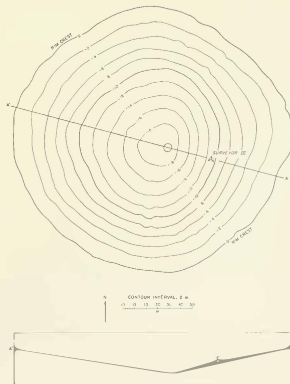
FIGURE 6-22.—Contour map and profile of crater in which Surveyor III landed.
