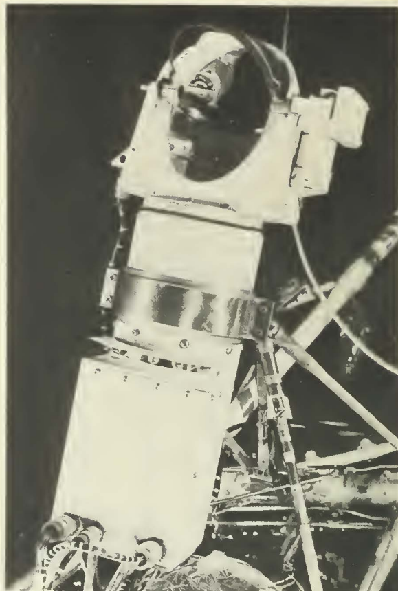
FIGURE 3-1.—Surveyor I television camera.
