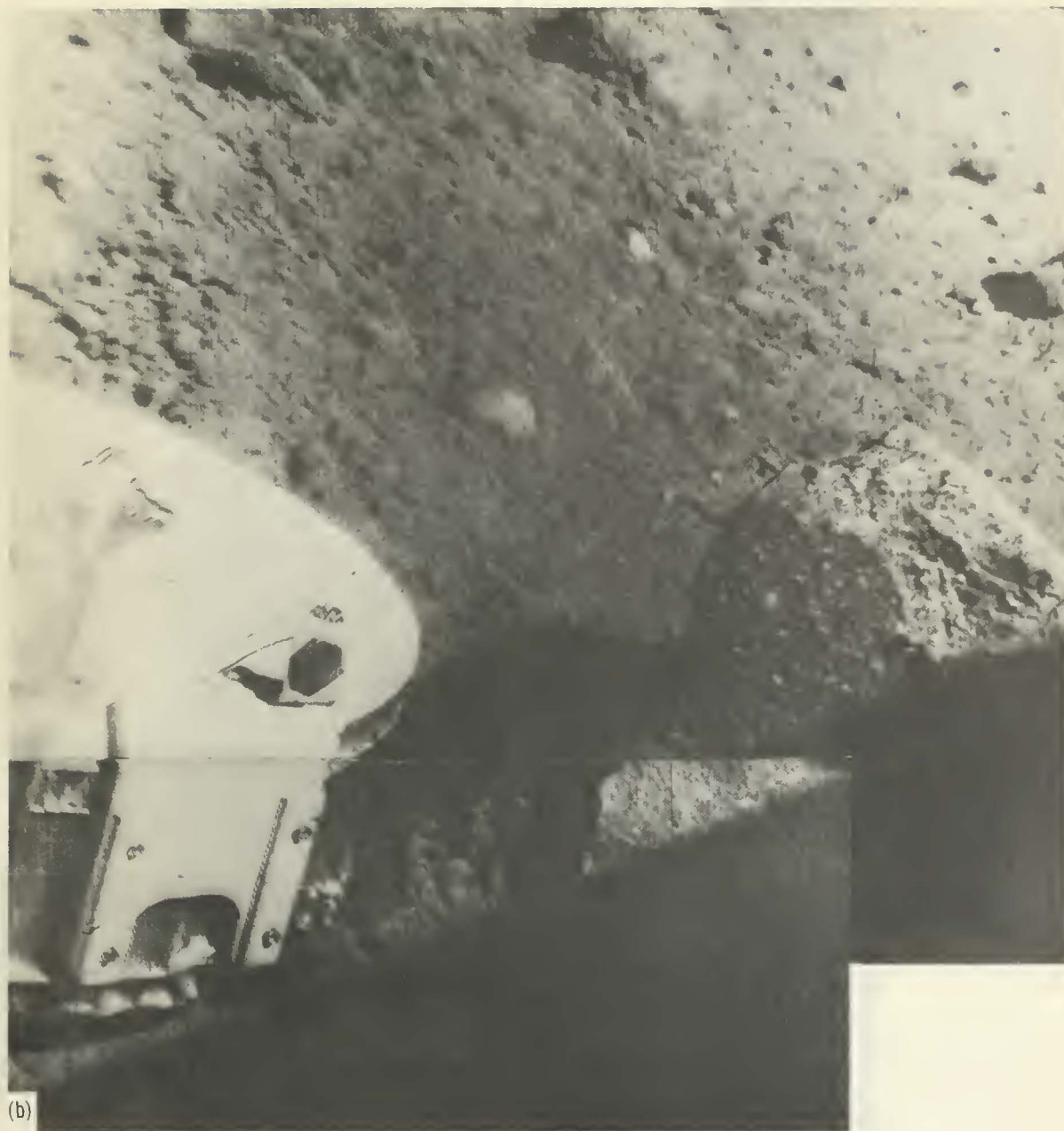
FIGURE 7-28.—Surveyor VII footpads after landing north of Tycho. (a) Footpad 2 (Catalog 7-SE-7). (b) Footpad 3. Because the penetration depths of the footpads were less than 6 cm, neither magnet contacted lunar surface material.
