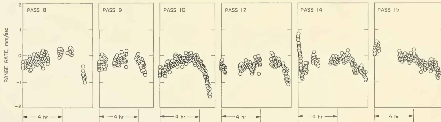
FIGURE 10-29.—Surveyor VI. Tracking passes of unbiased and biased data: DSS 42.
