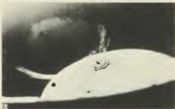
FIGURE 4-11.—Textural detail of footpad imprints. (a) Surveyor I footpad 2. Ejected soil clumps (which, for the most part, are larger than naturally occurring fragments adjacent to the footpad) demonstrate that the soil is cohesive (June 4, 1966, 06:55:26 GMT, computer processed). (b) Surveyor III footpad 2 imprint made during final landing has a waffle pattern impressed by the bottom of the footpad; low Sun angle illumination (Apr. 20, 1967, 09:05:17 GMT). (c) Surveyor III footpad 2 imprint as seen with high Sun angle illumination. Walls and bottom of imprint have higher reflectivity than natural undisturbed lunar surface. Flat surfaces and shapes of many fragments on near side of imprint indicate that the fragments have been only slightly displaced (Apr. 26, 1967, 06:05:55 GMT). (d) Surveyor V part of trench wall formed by footpad 2; cohesion permits soil to stand at angles greater than the angle of repose of loose material (Sept. 14, 1967, 04:42:06 GMT). (e) Surveyor VI footpad 2 imprint made during initial landing, showing compressed soil in imprint wall and floor (Nov. 16, 1967, 03:35:09 GMT). (f) Surveyor VI footpad 2 imprint made during hop. The smoothness of the imprint wall demonstrates the fine-grained nature of lunar soil. Particles are smaller than the
