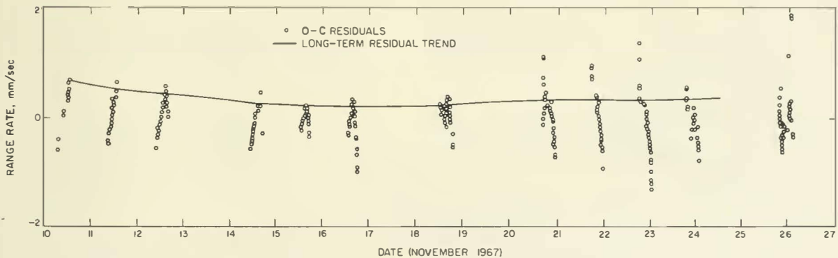
FIGURE 10-5.—Surveyor VI, DSS 42. First lunar day, O—C residual set (compressed five data points/min). LE 5 was used.
