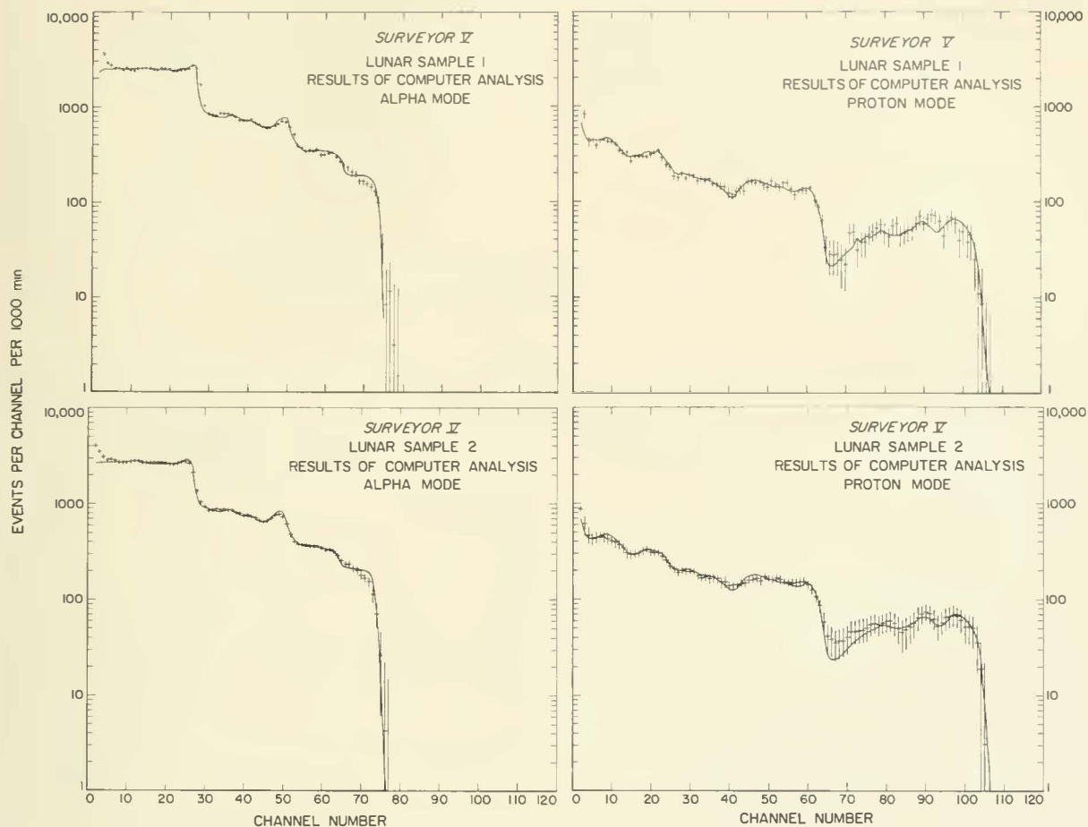
FIGURE 8-35.—Computer analyses of the Surveyor V lunar sample spectra. Comparison between the calculated spectra (smooth curves), using an eight-element library, and the data obtained on the lunar surface (after background subtraction).
