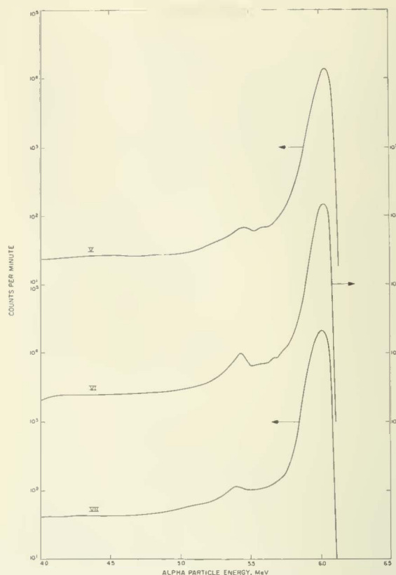
FIGURE 8-14.—Composite energy spectra for each of the three sets (six sources each) of the curium-252 flight sources.
