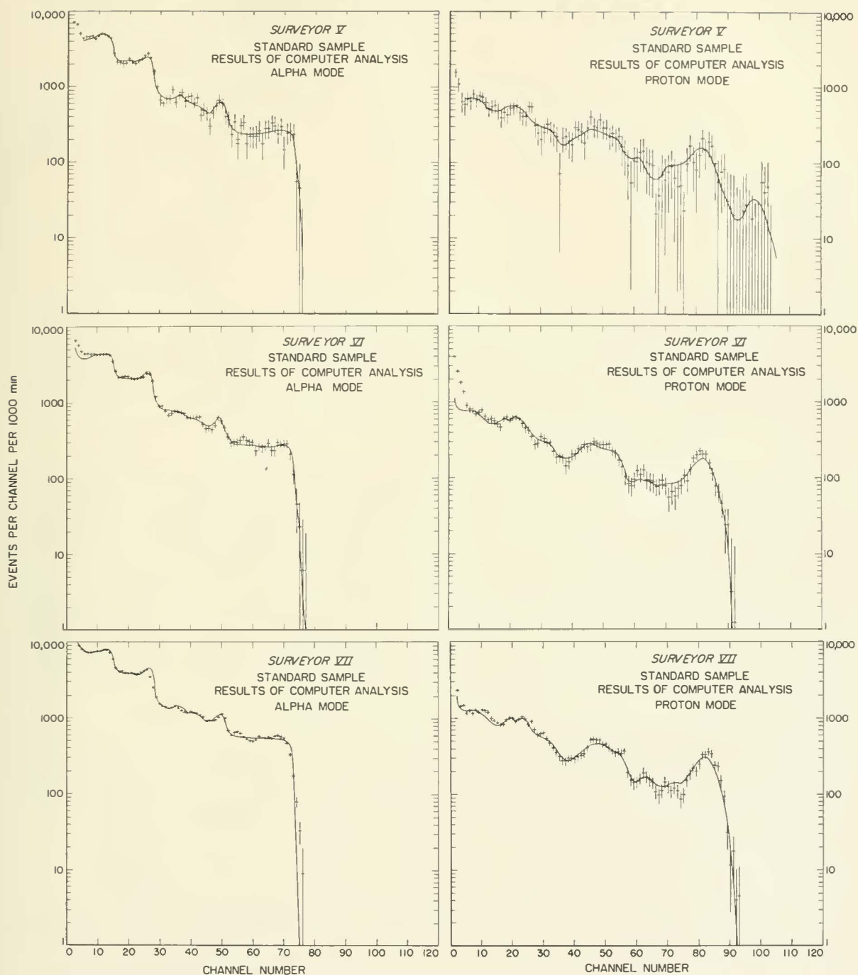
FIGURE S-30.—Computer analyses of the Surveyor standard sample spectra. Comparison between the calculated spectra (smooth curves), using an eight-element library, and the data obtained on the Moon (after background subtraction).
