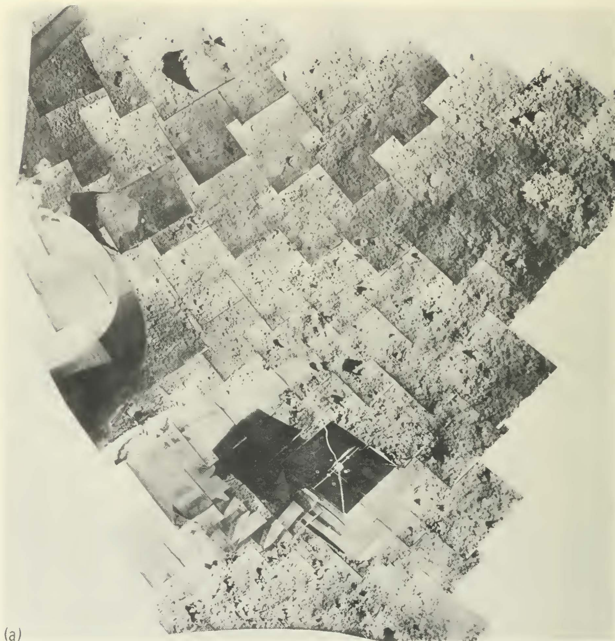
FIGURE 8-25.—(a) High-resolution mosaic of the Surveyor V sensor head on the lunar surface before vernier firing (Sept. 12, 1967, Catalog 5-MP-24). (b) Mosaic after vernier firing (Sept. 14, 1967, Catalog 5-MP-25).
