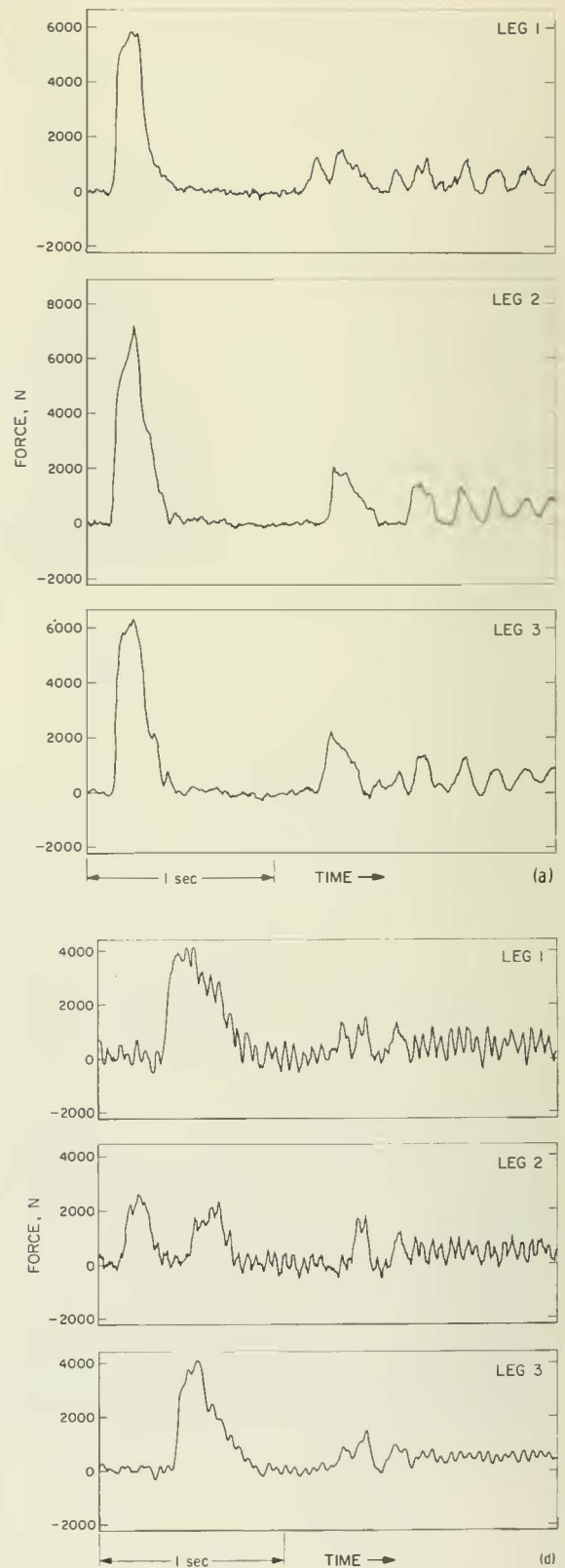
FIGURE 4-4.—Telemetry data showing initial shock-absorber axial load histories during Surveyor landings. In most cases, oscillations continue beyond the 2.5 seconds shown. (a) Surveyor I: landing. (b) Surveyor III: first touchdown. (c) Surveyor III: second touchdown. (d) Surveyor III: final landing. (e) Surveyor V: landing. (f) Surveyor VI: initial landing. (g) Surveyor VI: hop landing. (h) Surveyor VII: landing.
