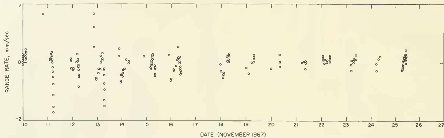
FIGURE 10-26.—Surveyor VI, DSS 11. First lunar day, O—C residual set (compressed five data points/min). LE 5 was used.
