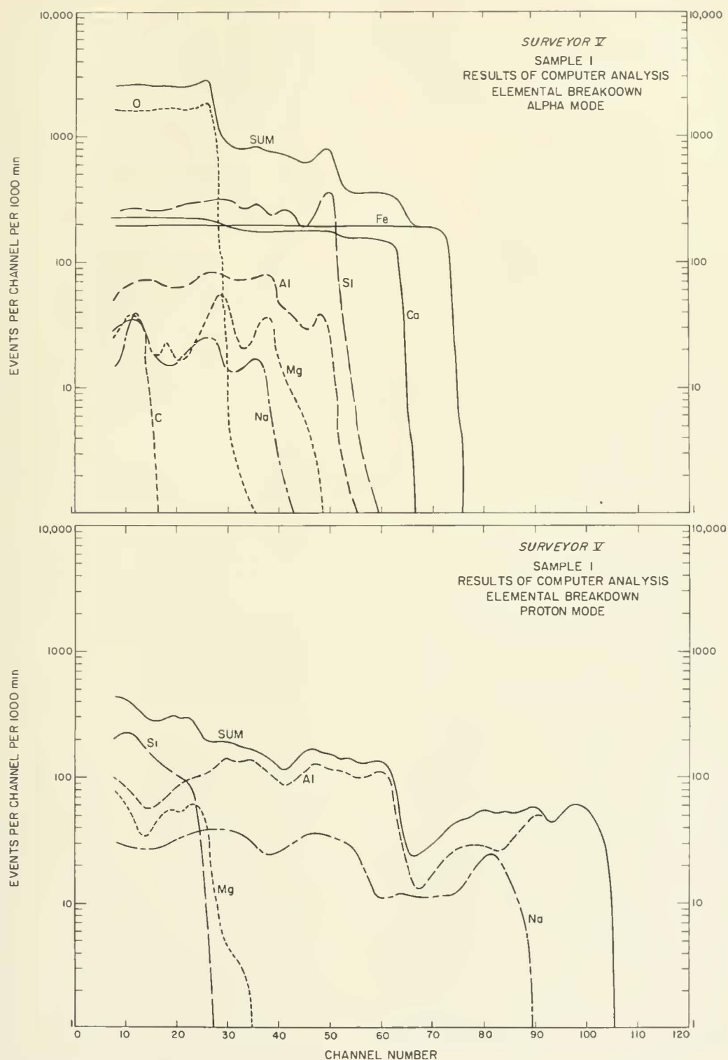
FIGURE S-37.—Contribution of separate elements to least-squares computer analysis of the Surveyor V spectra from lunar sample 1. The library data for the separate elements are shown in the relative amounts needed to explain the observed lunar data.
