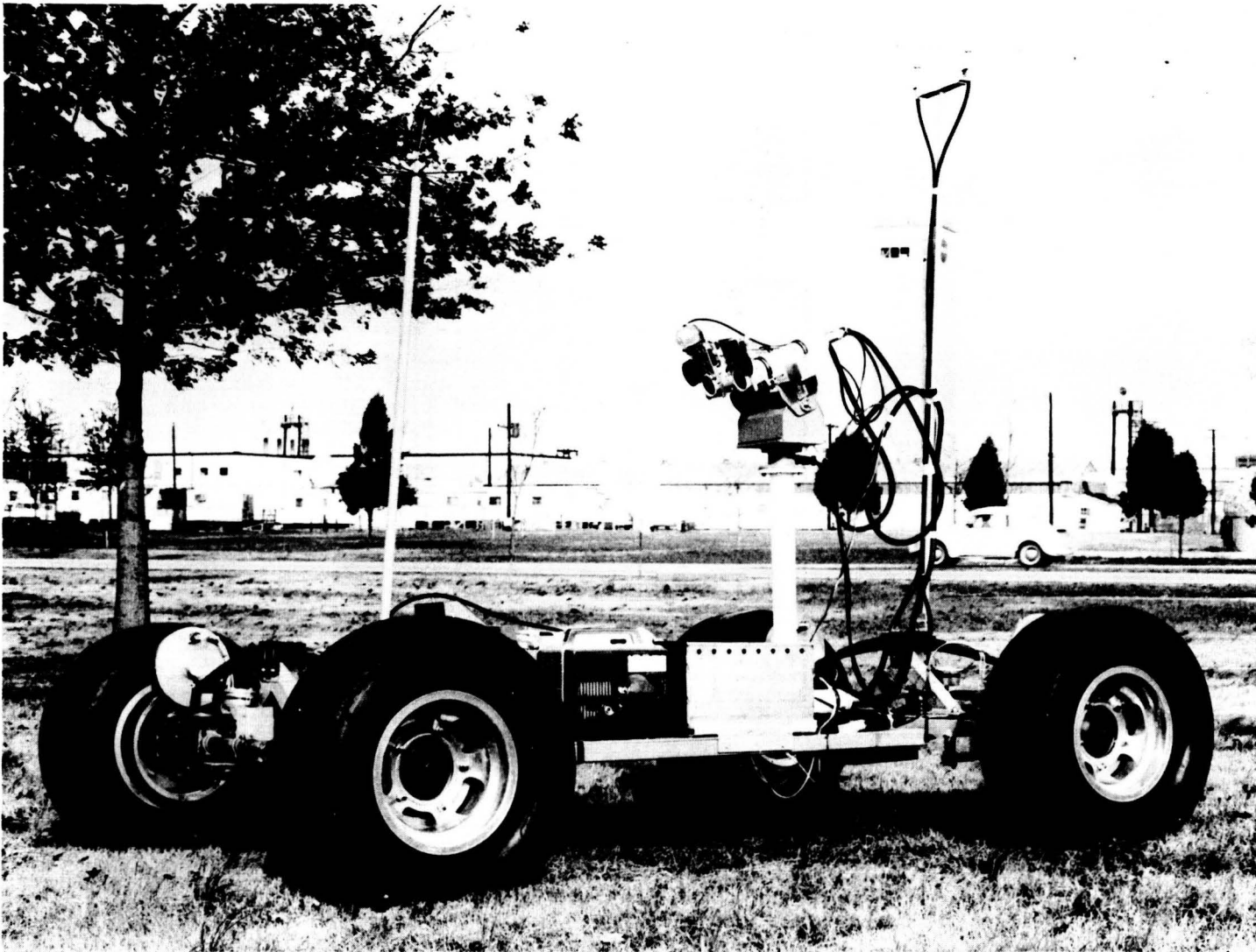
Figure 2. Breadboard vehicle with remote control operations.
