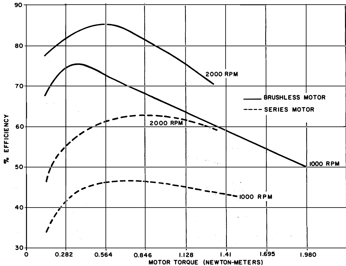
Figure 12. Efficiency vs torque
