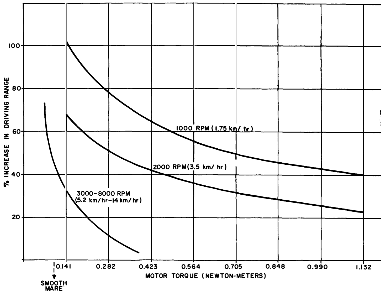
Figure 13. Percent increase in driving range of brushless motor over series motor as a function of torque.
