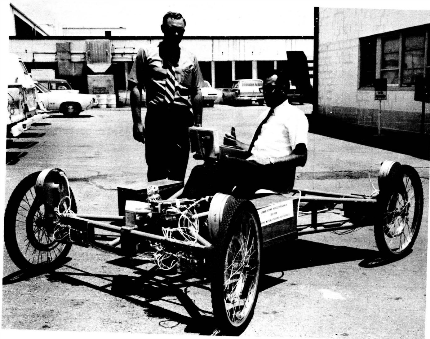
Figure 1. Breadboard vehicle.
