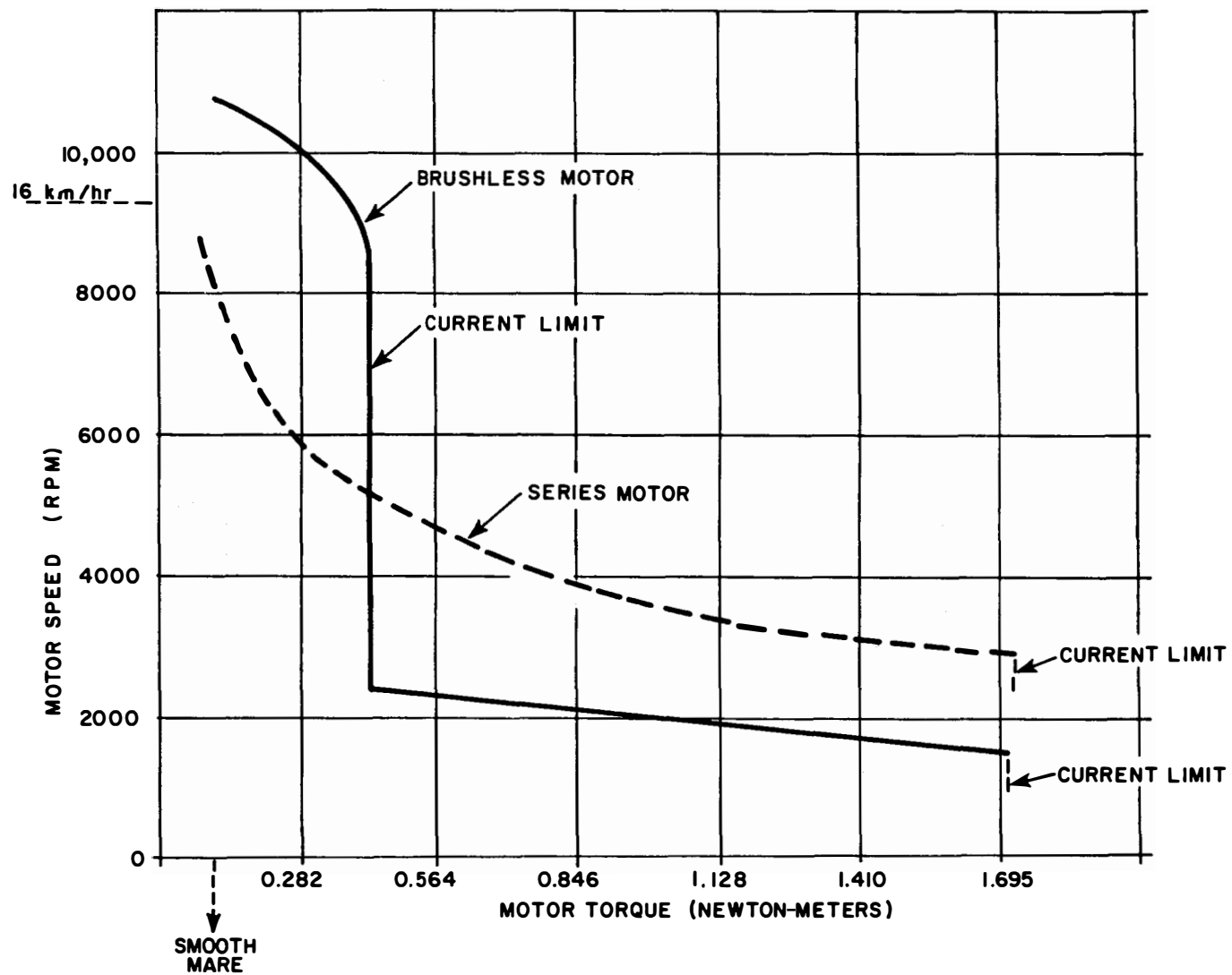
Figure 10. Torque vs speed maximum performance curves.
