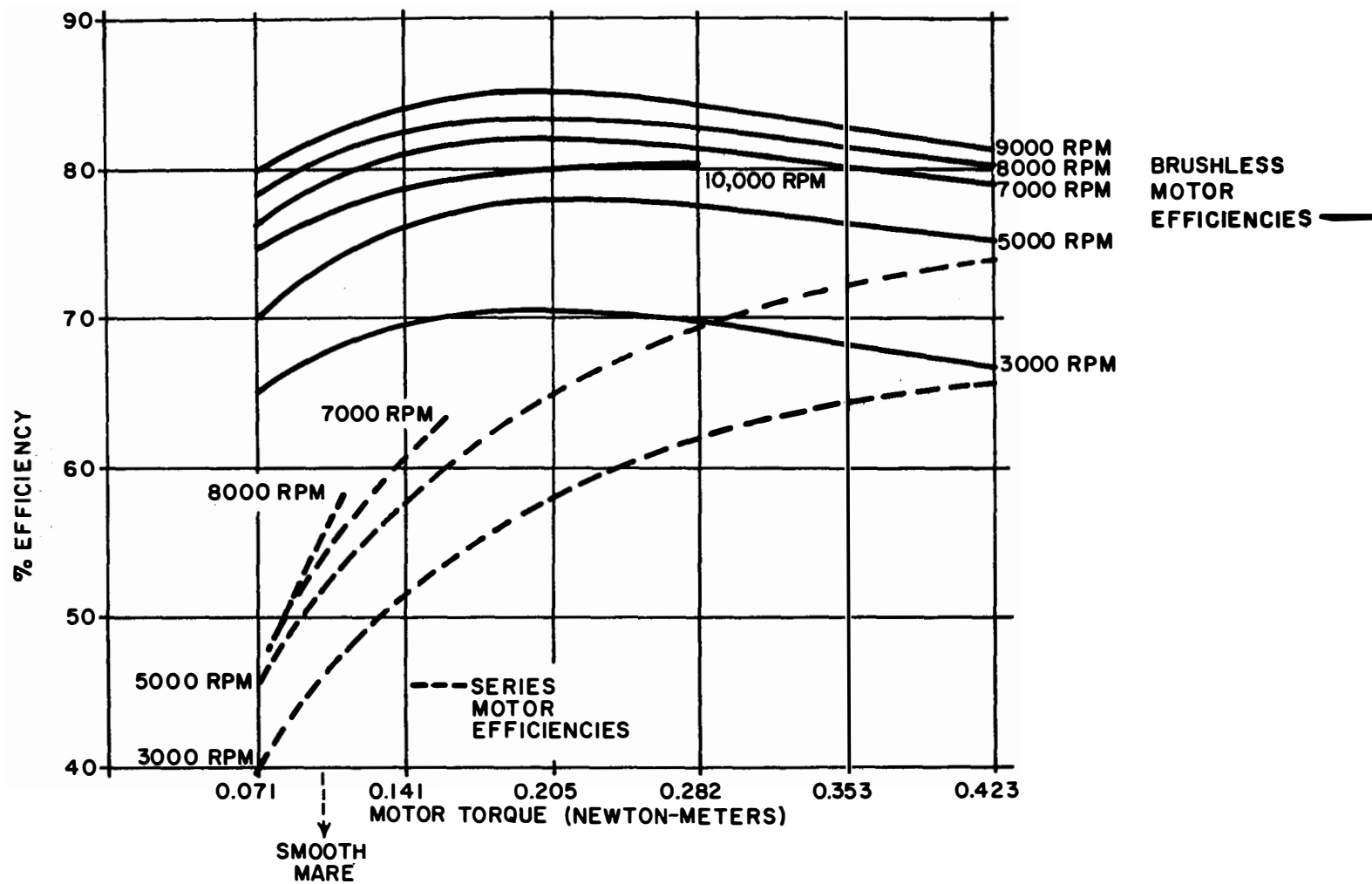
Figure 11. Efficiency vs torque.
