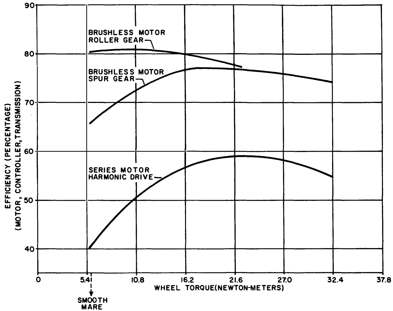
Figure 15. Efficiency vs torque for maximum torque speed.
